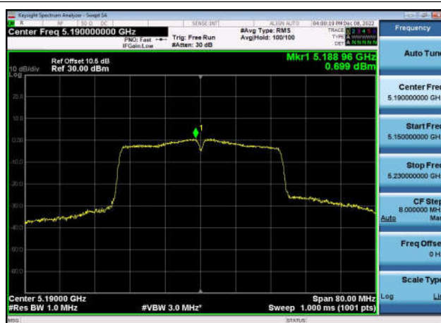
U-NII-1 Power spectral density-802.11 ac(40MHz),5190MHz,Ant1
