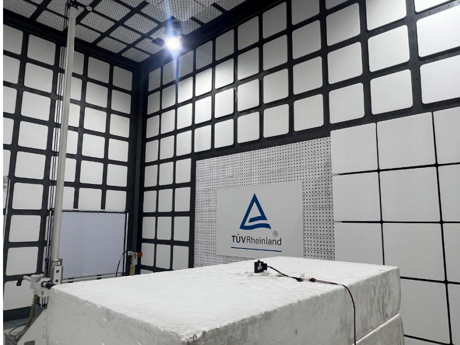
Photograph 7: Test Setup for Spurious Emissions (Back View 3)
