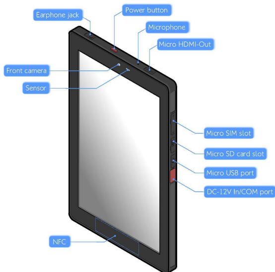
Figure 1: Top and Right panel of the VIEGA tablet
