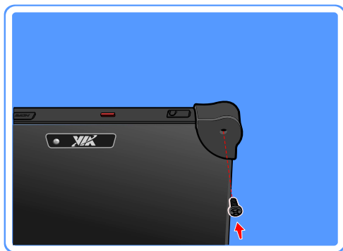
Figure 12: Secure the rubber ribs
