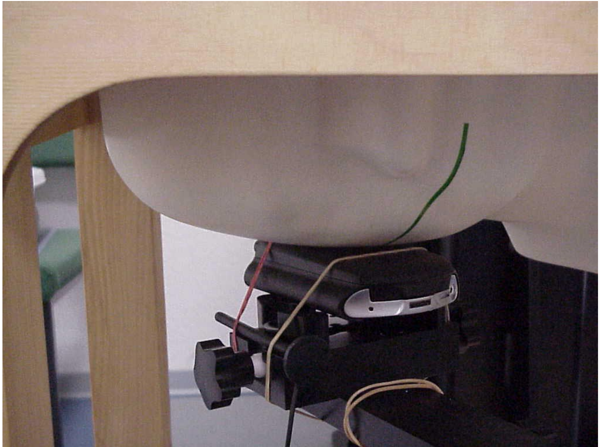
Photo 3: Position cheek15° (head SAR measurement)
