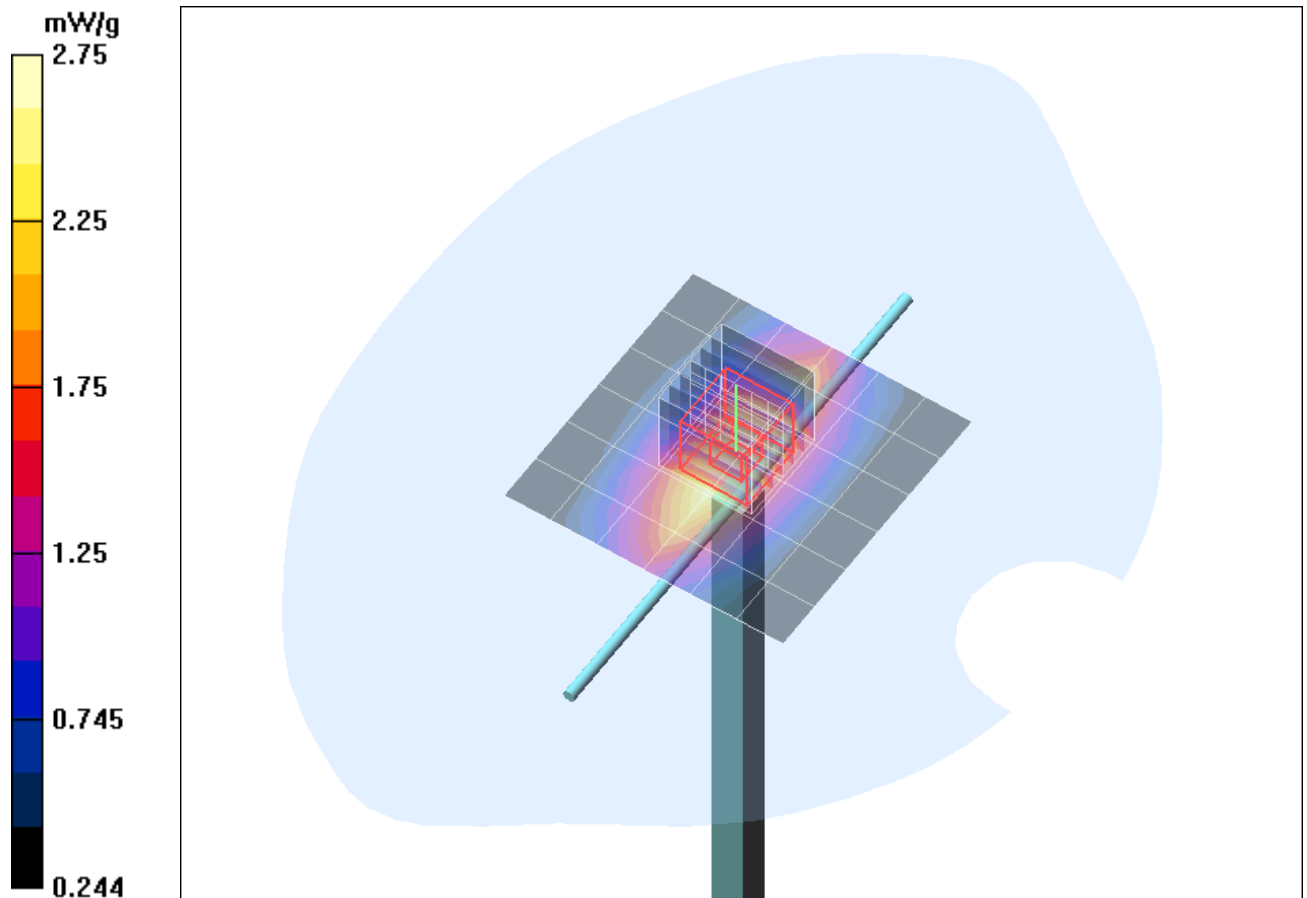
Fig. 11: Validation measurement 835 MHz Body (GPRS/EDGE 850, July 28, 2011), coarse grid. Ambient Temperature: 22.8°C. Liquid Temperature: 22.3°C.
