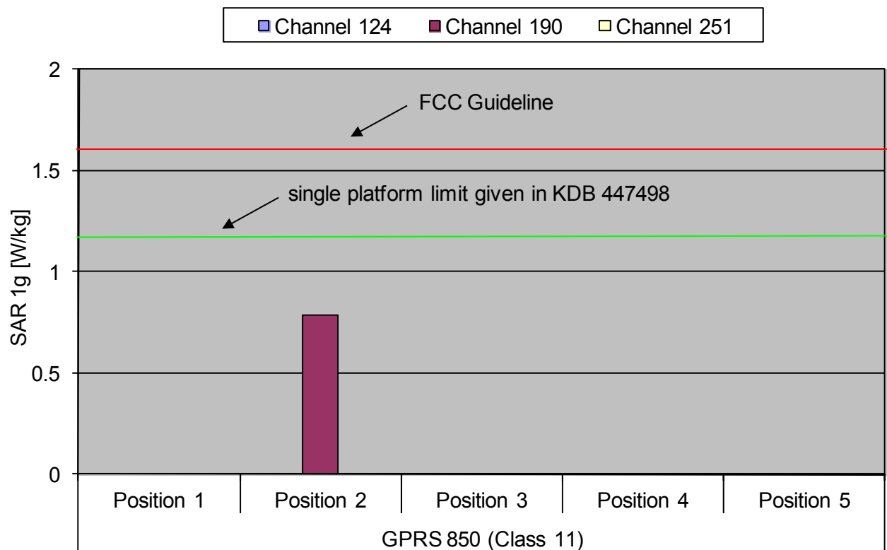
Fig. 6: The measured SAR values for the Option GI0644 for GPRS 850 (Class 11) in comparison to the FCC exposure limit.
