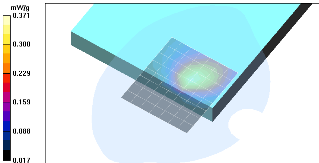
Fig. 6: SAR distribution for GSM 850, channel 190, Packard Bell Easy Note, position 1. (29.11.2004; Ambient Temperature: 21.2° C; Liquid Temperature: 20.6° C).
