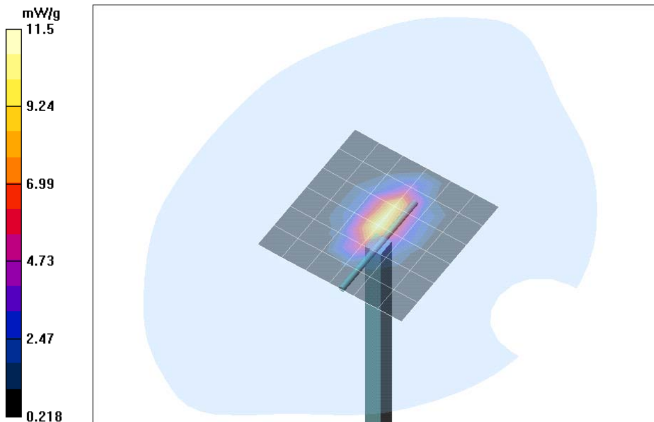
Fig. 15: Validation measurement 1900 MHz Body (December 01, 2004), coarse grid. Ambient Temperature: 22.0° C, Liquid Temperature: 21.0° C.
