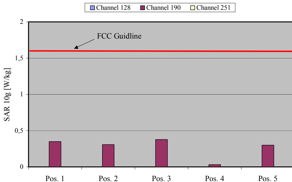
Fig. 9: The measured SAR values for the Option Magnum Lite Card in combination with a Packard Bell Easy Note Notebook for GPRS 850 in comparison to the FCC exposure limit.
