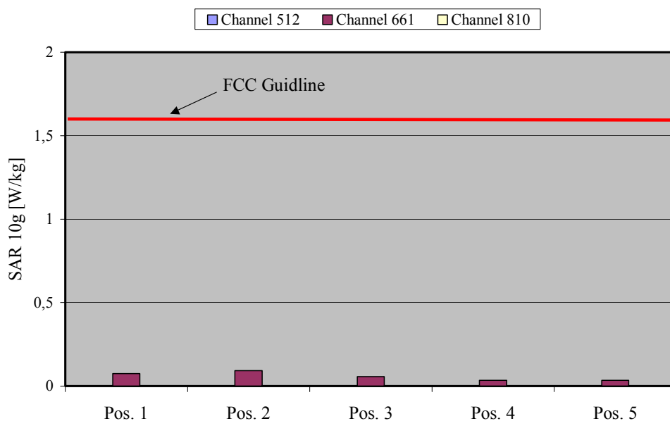
Fig. 11: The measured SAR values for the Option Magnum Lite Card in combination with a DELL Latitude D505 Notebook for GPRS 1900 in comparison to the FCC exposure limit.
