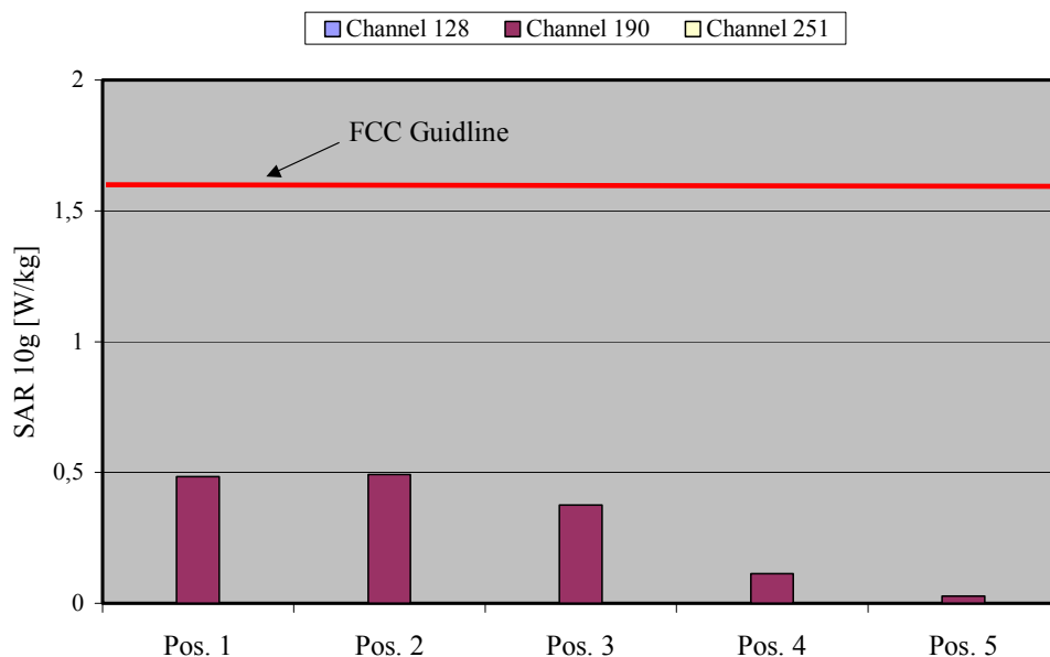
Fig. 8: The measured SAR values for the Option Magnum Lite Card in combination with a DELL Latitude D505 Notebook for GPRS 850 in comparison to the FCC exposure limit.
