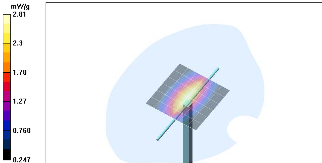
Fig. 14: Validation measurement 835MHz Body (November 29, 2004), coarse grid. Ambient Temperature: 22.0° C, Liquid Temperature: 21.0° C.
