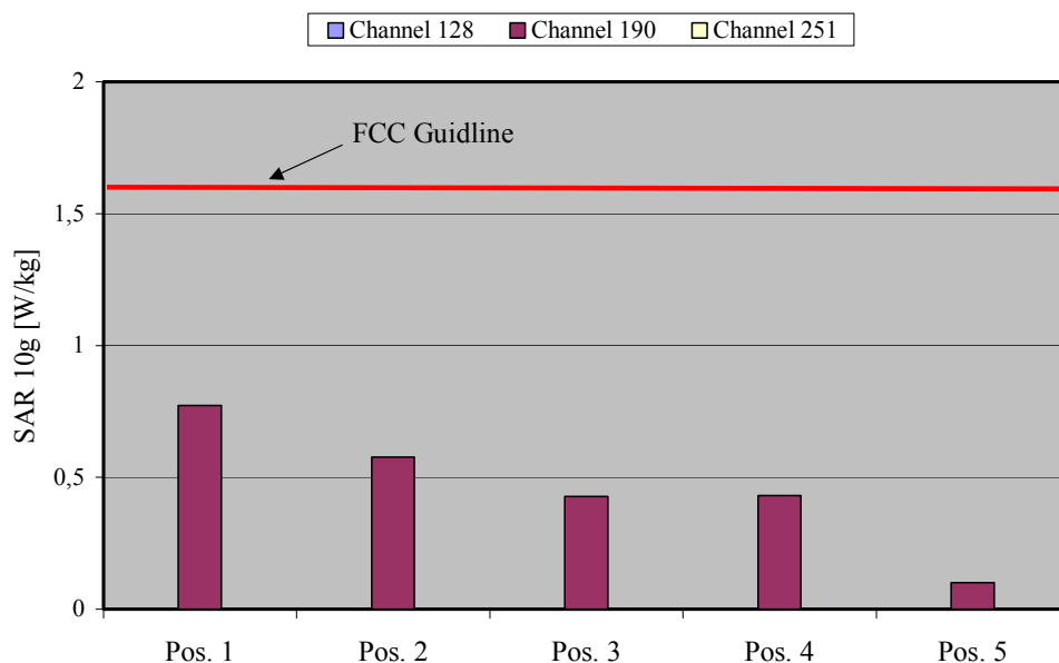
Fig. 10: The measured SAR values for the Option Magnum Lite Card in combination with a Acer Aspire 2020 Notebook for GPRS 850 in comparison to the FCC exposure limit.
