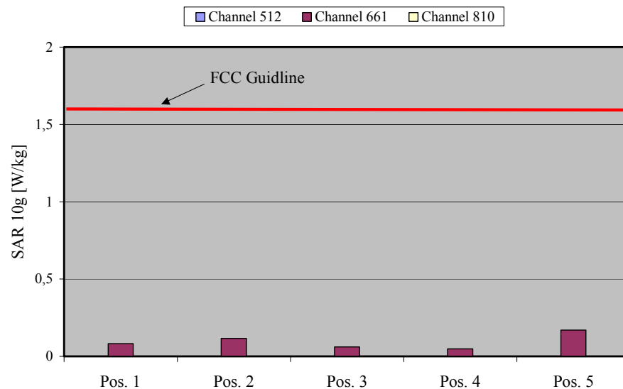
Fig. 12: The measured SAR values for the Option Magnum Lite Card in combination with a Packard Bell Easy Note Notebook for GPRS 1900 in comparison to the FCC exposure limit.
