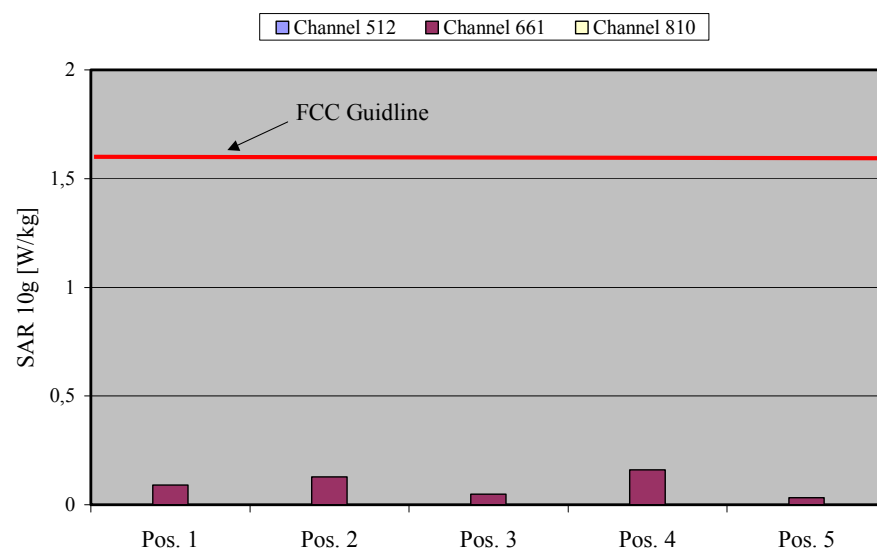
Fig. 13: The measured SAR values for the Option Magnum Lite Card in combination with a ACER Aspire 2020 Notebook for GPRS 1900 in comparison to the FCC exposure limit.
