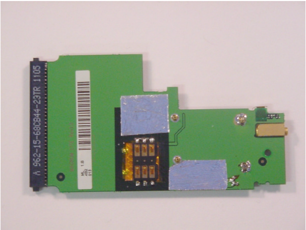
Photo 3: EUT (rear side, without housing)
