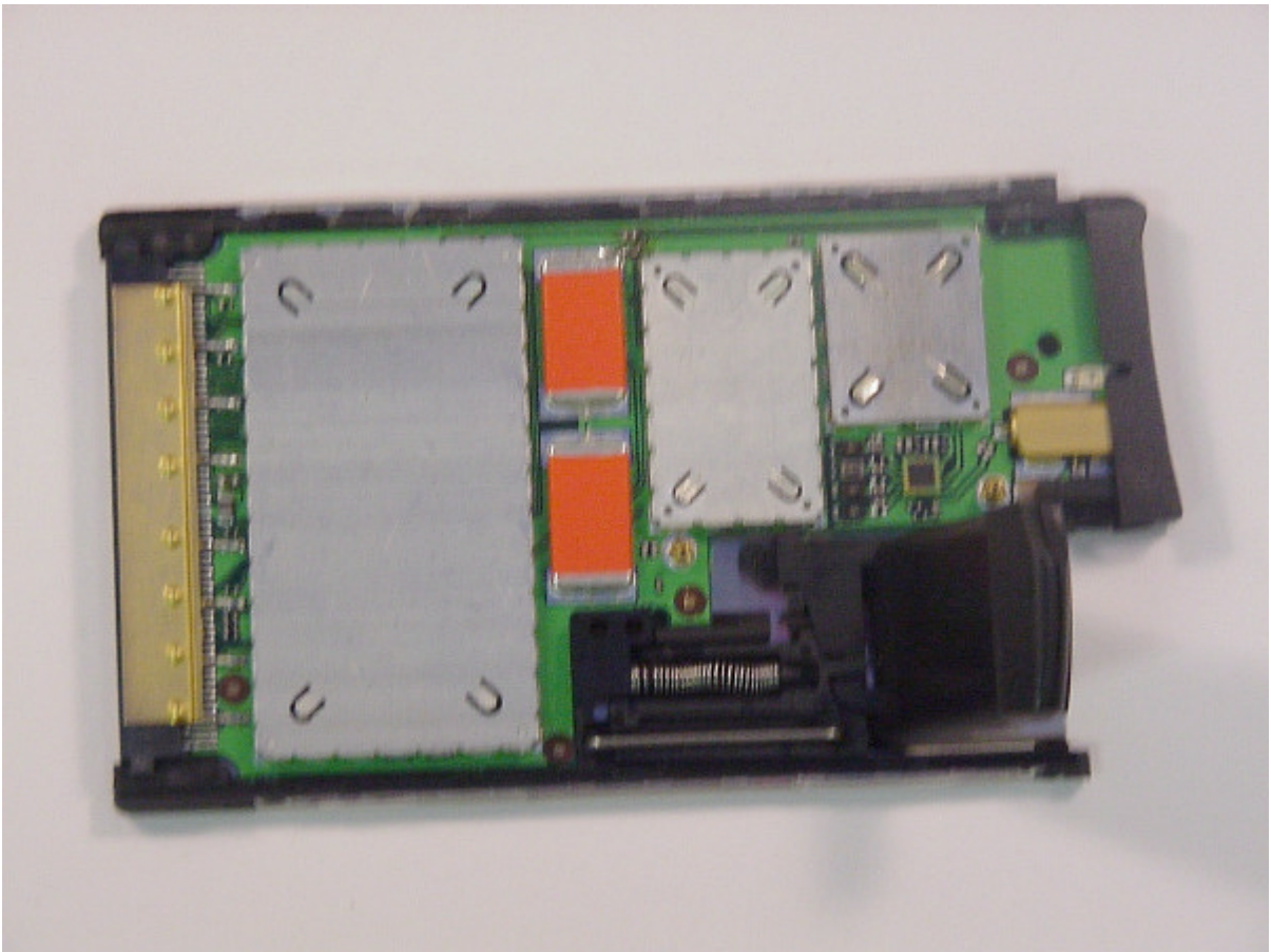
Photo 2: EUT (topside, without housing)
