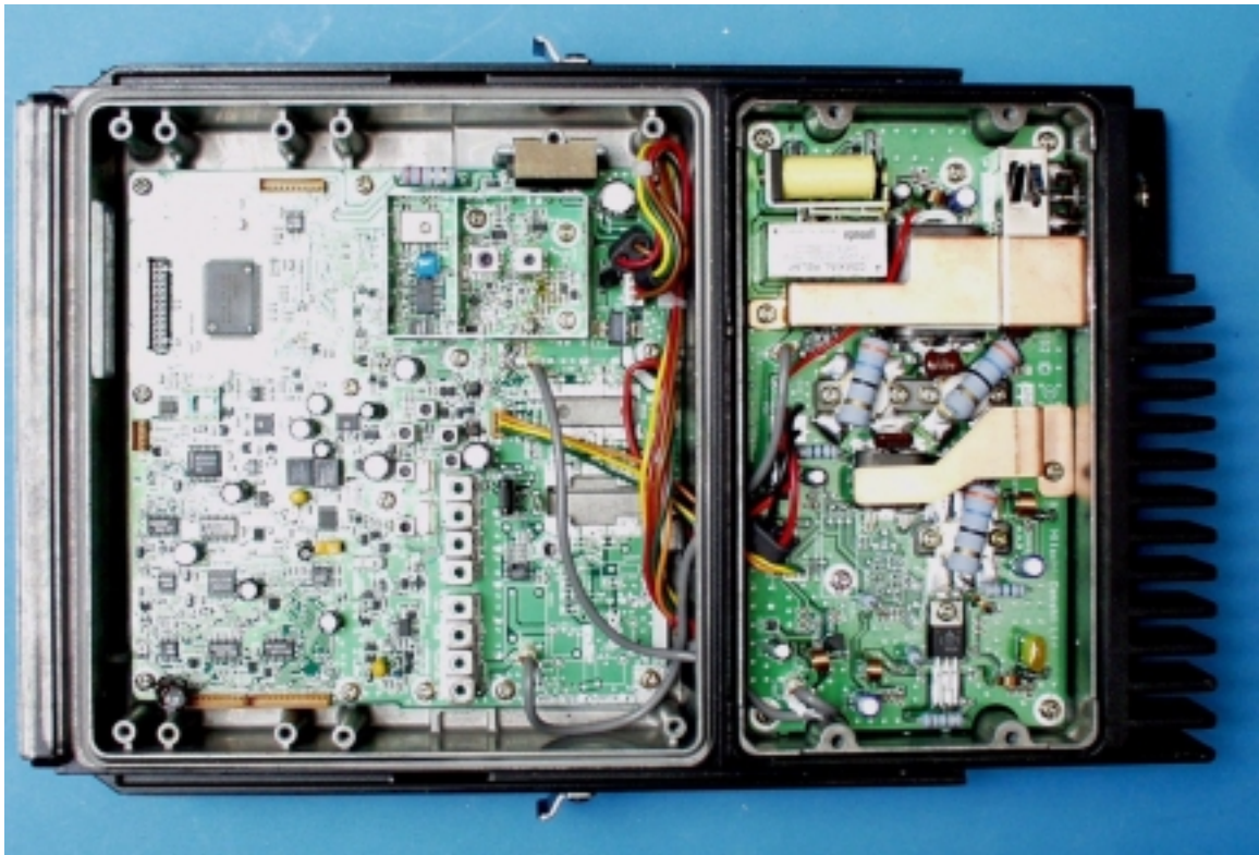
COMPONENT WITH SHIELDS
