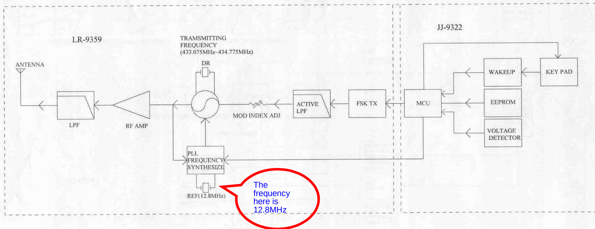
TRANSMITTER FUNCTION BLOCK
