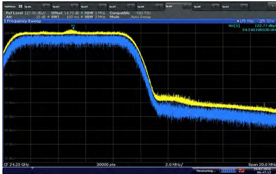
High Channel Band-Edge using 1MHz RBW/3MHz VBW
