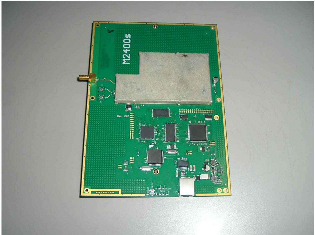
PCB Back with Internal Shield Installed:
