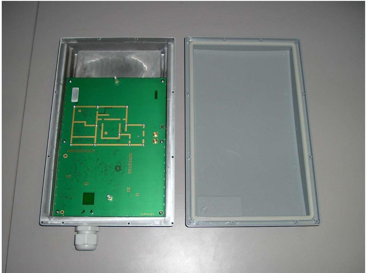
PCB in Shield and Radome:
