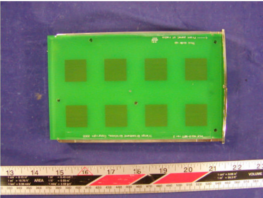
Transceiver – Top View
