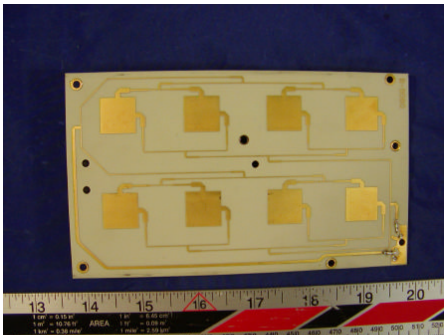
Transceiver – Board Bottom and Antenna
