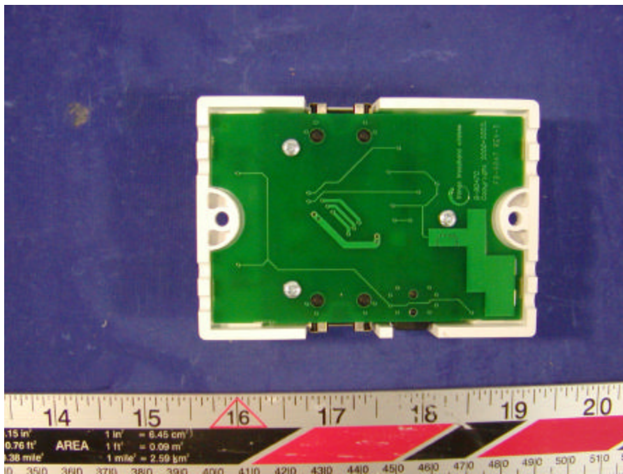
J Box – Bottom View
