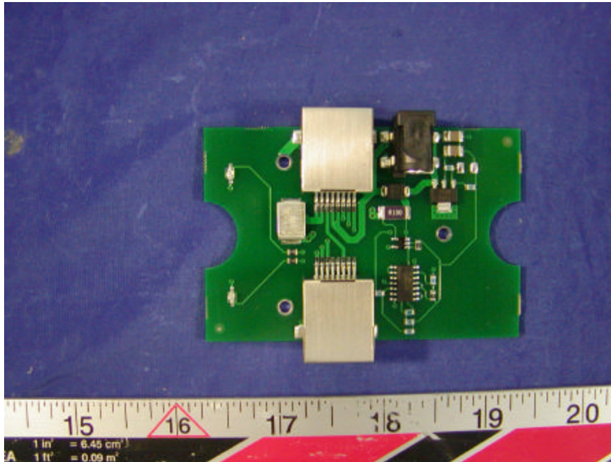
J Box – Board Component View
