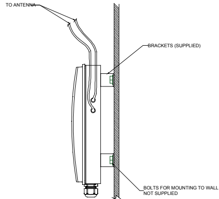
WALL MOUNTING
