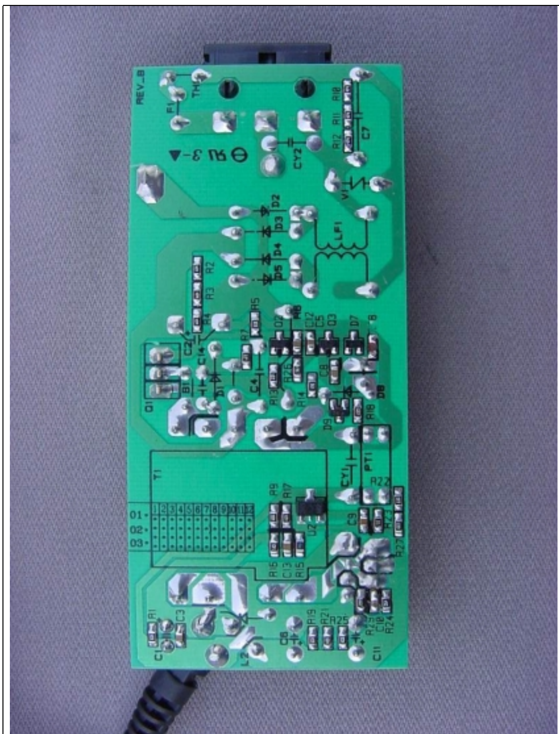
[ Bottom View of the Power Board in an AC/DC Adaptor ]
