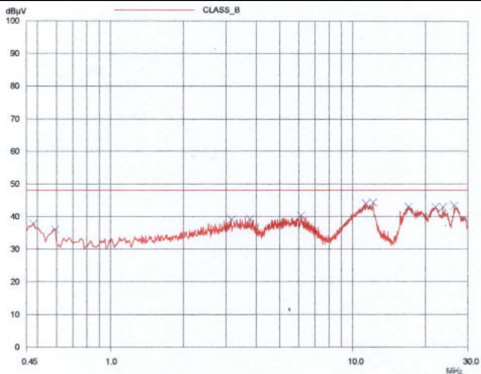
NEUTRAL LINE
