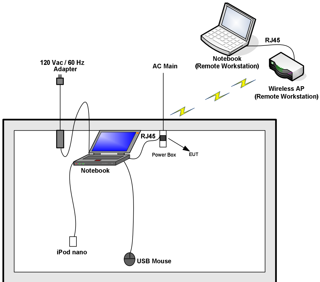
Test Setup Diagram - Radiated Test (Below 1GHz)
