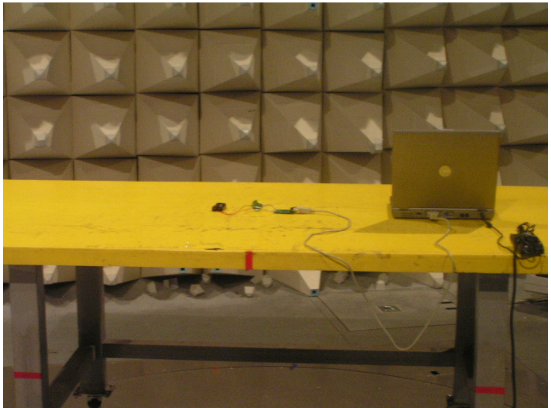
REAR VIEW
