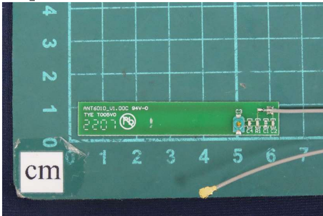
(27) EUT Photo_NFC Antenna: Sunion / ANT-6010-IPX110
