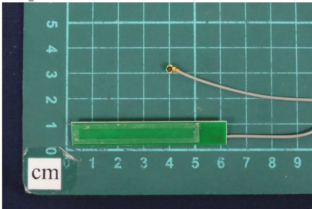
(28) EUT Photo_NFC Antenna: Sunion / ANT-6010-IPX110
