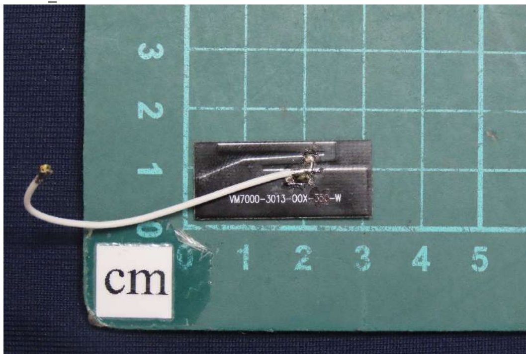
(31) EUT Photo_RF Antenna: Vicmoor / VM7000-3013-OOX-65-W
