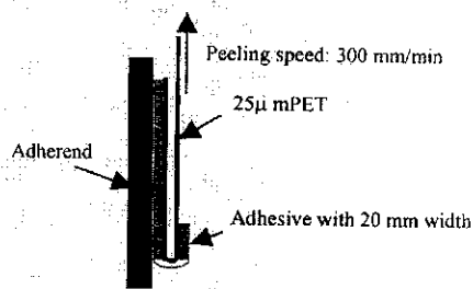
Fig. 1 Measurement method of 180° peeling
