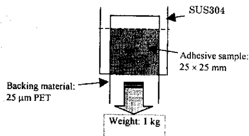
Fig. 2 Measurement method of holding power
