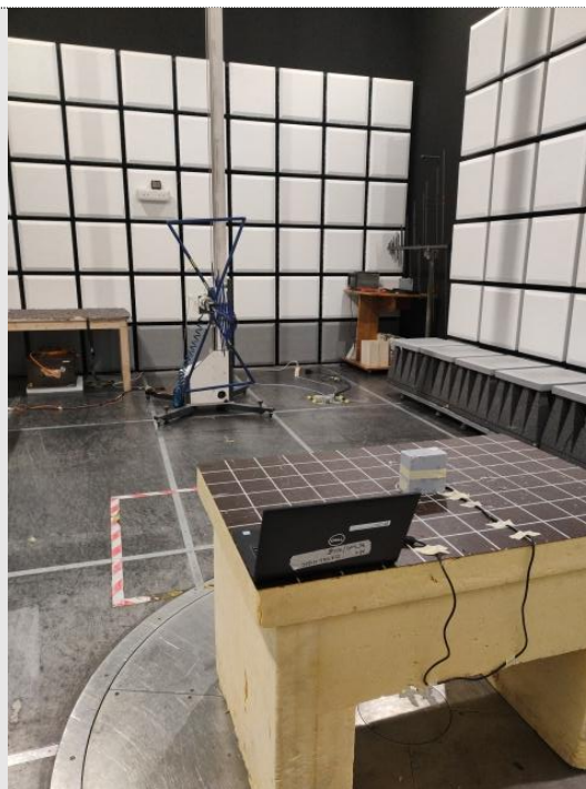
PHOTO N°2 - RADIATED EMISSION TEST SETUP
