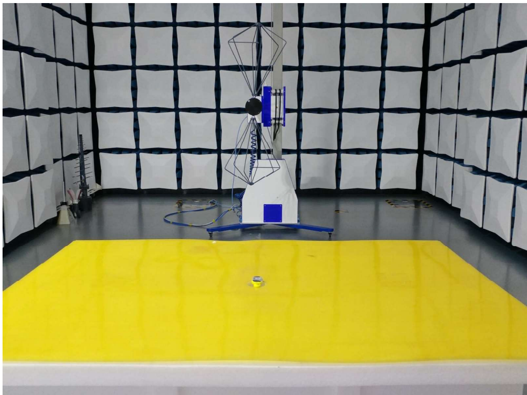
Set-up for Radiated Emission Below 1GHz
