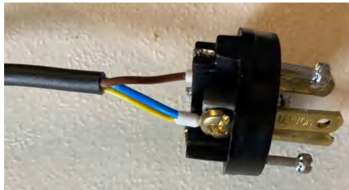
Example of a power plug wired for use in North America
