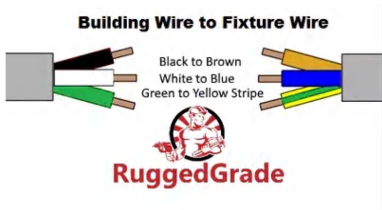
Example of how to wire a power plug for use in North America
