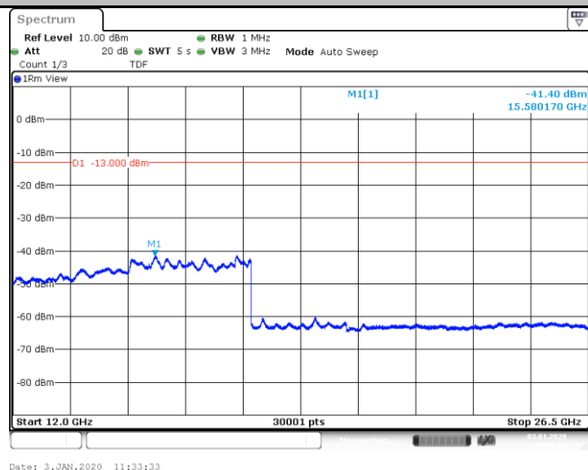
Band4_1.4MHz_QPSK_19957_1_0_Low_12000_26500_-41.4_PASS__
