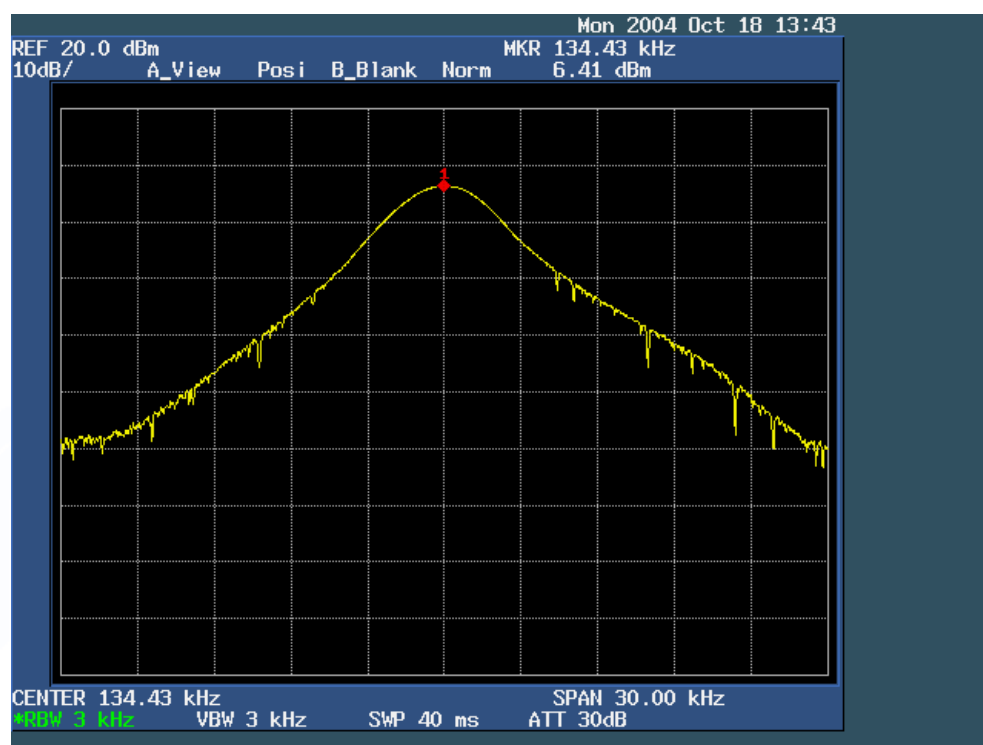
Emission Bandwidth plot
