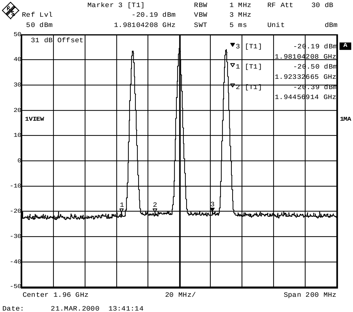
Fig. 43 – Slow frequency hopping – RBW = 1 MHz
