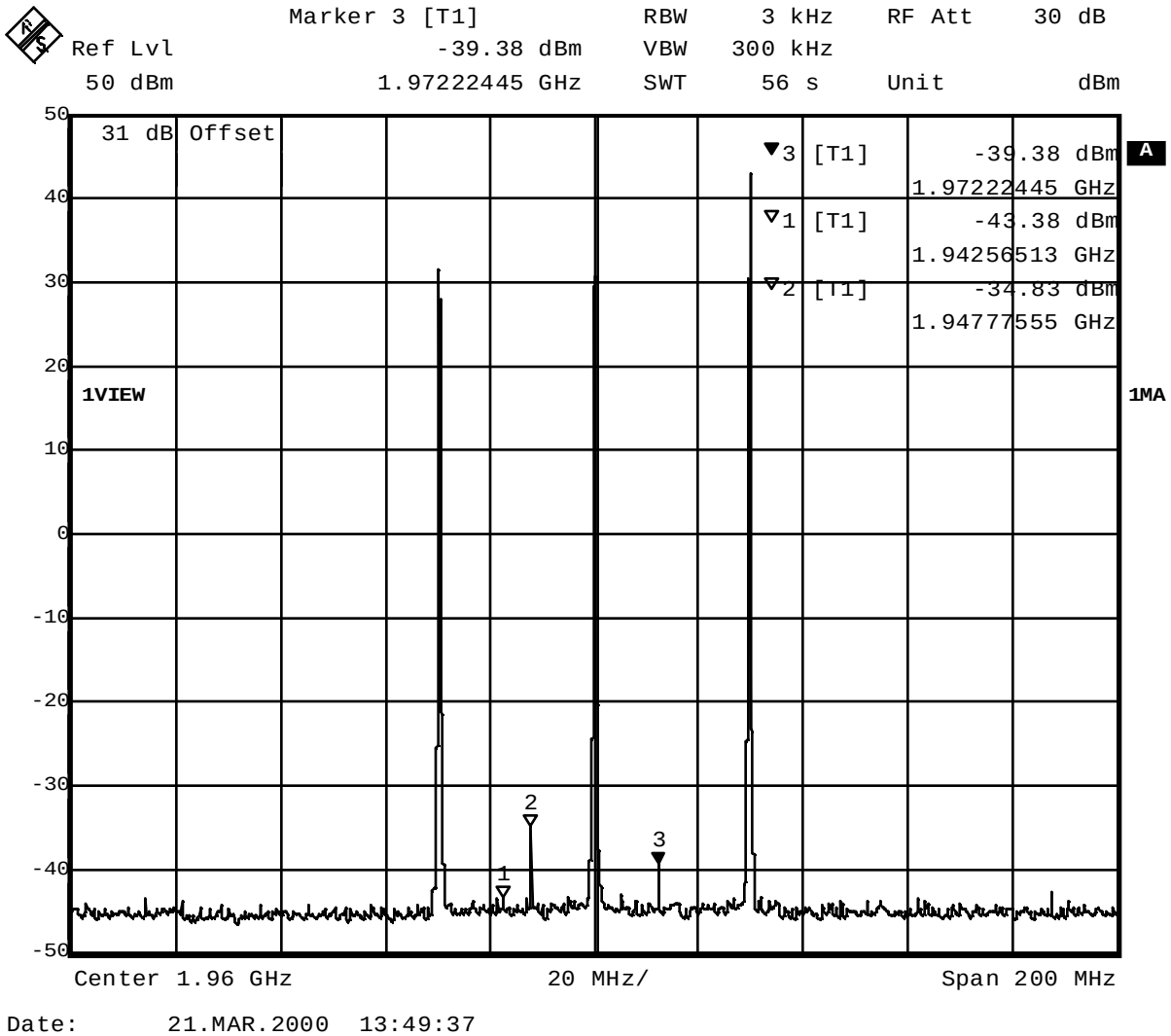
Fig. 46 – Slow frequency hopping – RBW = 3 kHz, reduced video bandwidth VBW = 300kHz.
