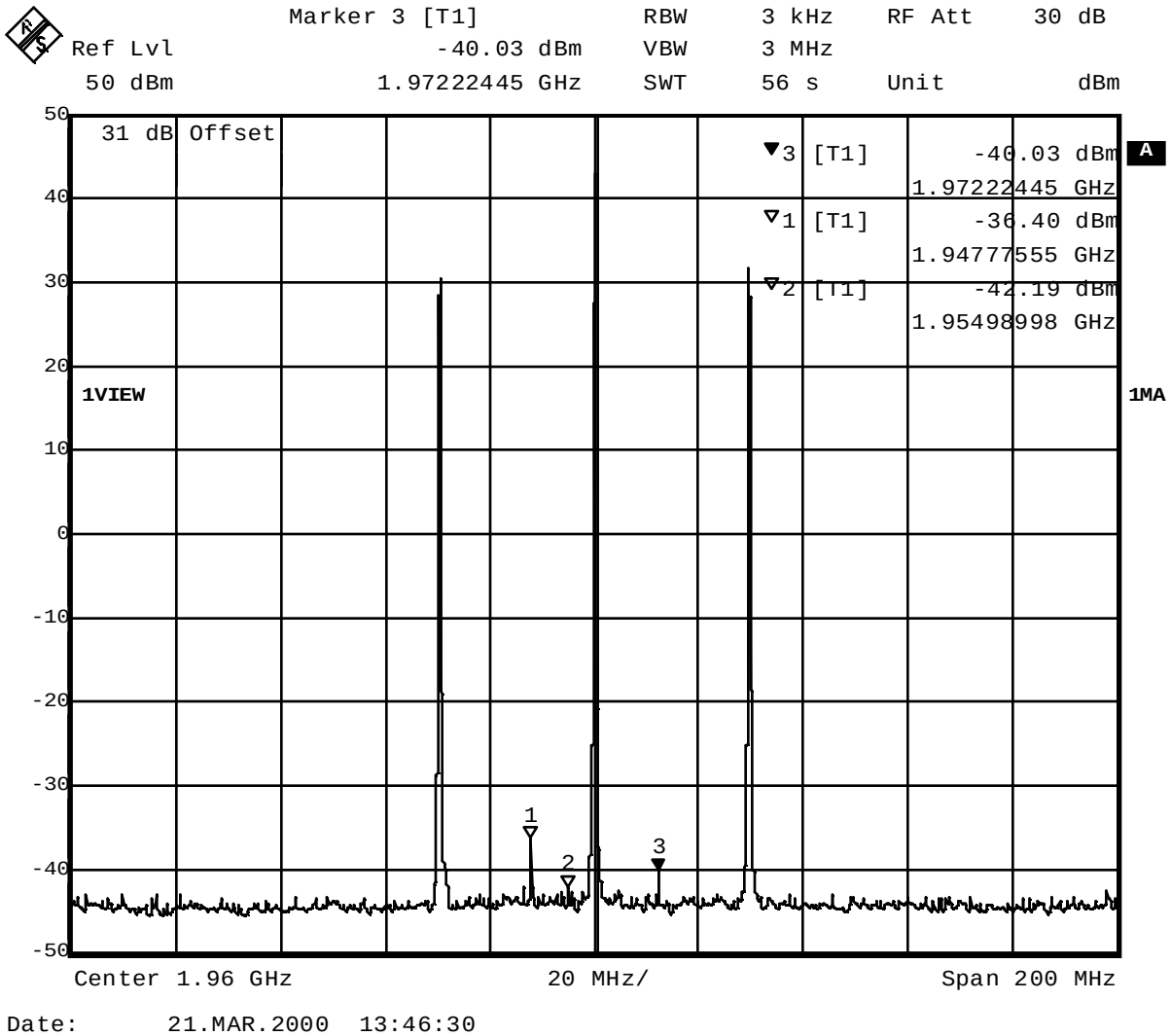
Fig. 45 – Slow frequency hopping – RBW = 3 kHz
