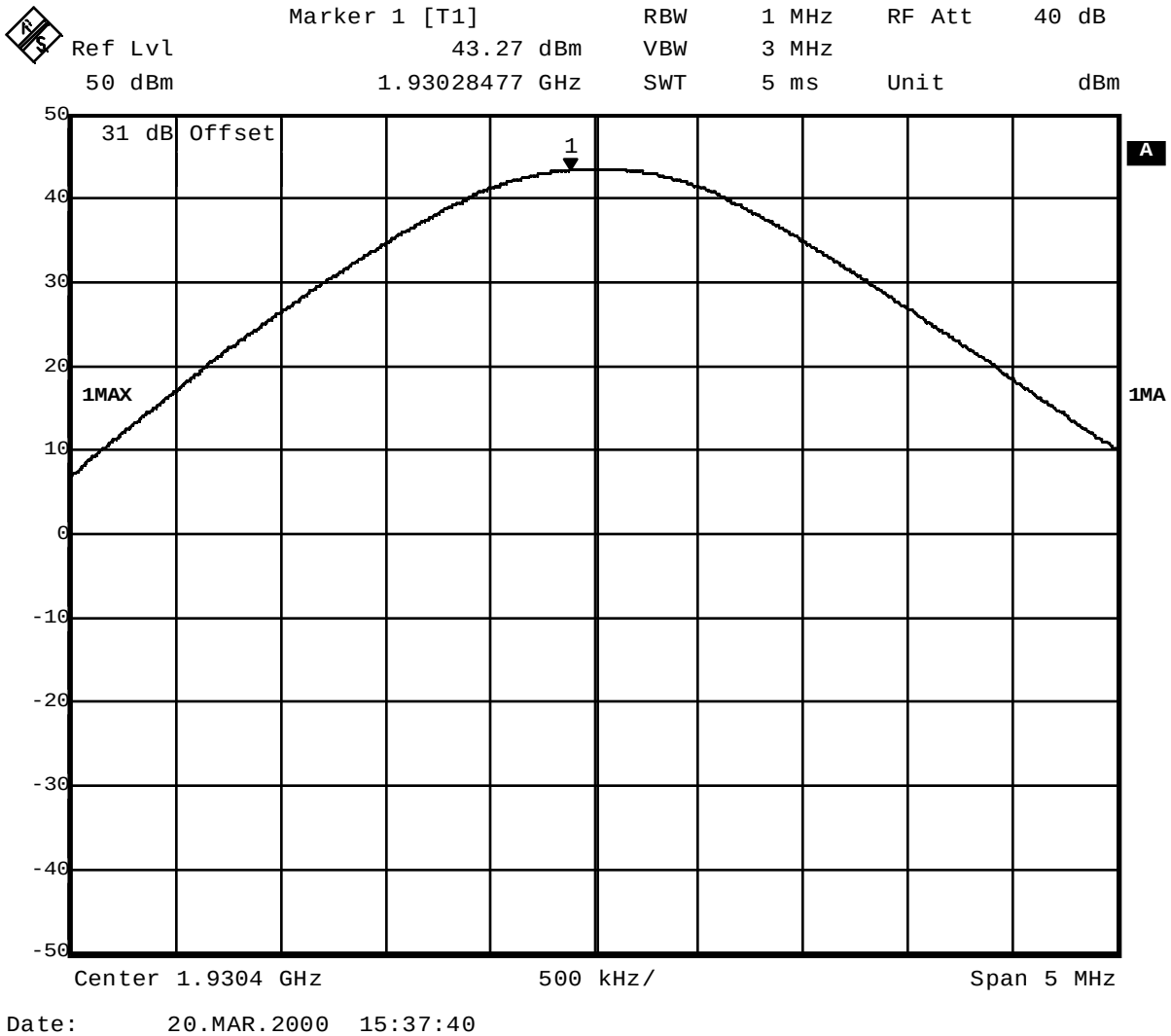
Fig. 3 – RF power at the antenna connector.
