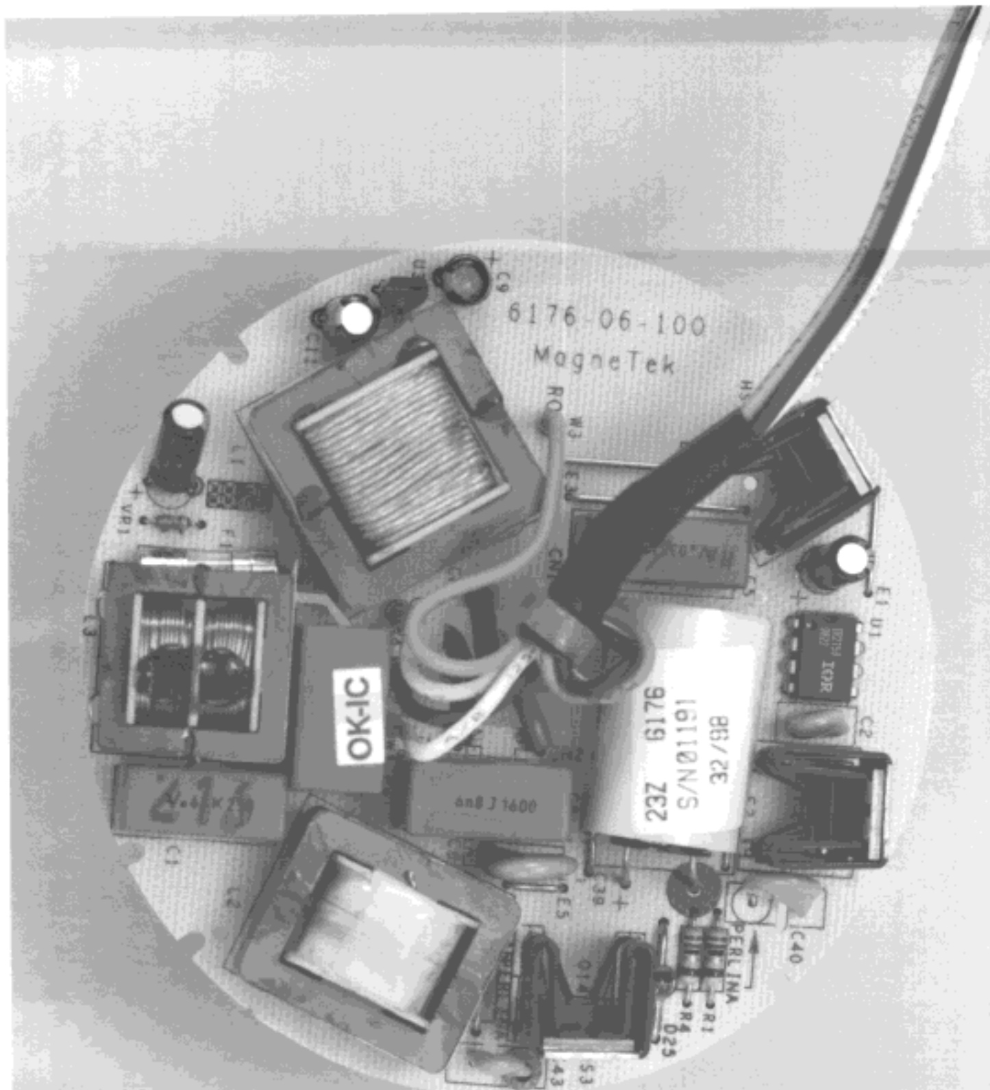
Exhibit G#1A Component Placement Model # FEH552D/HPF/DV/120 FCC ID: NE455DVHC
