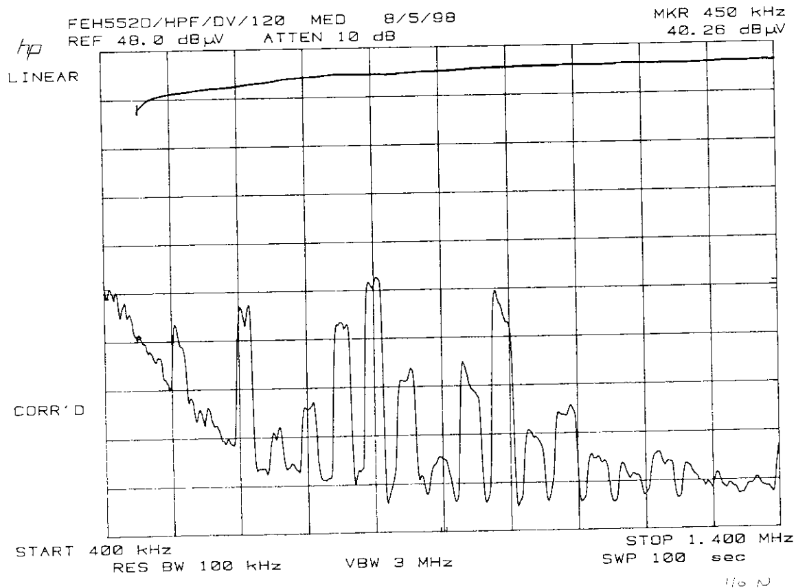
Fig. 8 CONDUCTED EMISSIONS MAGNETEK FEH552D/HPF/DV/120 FCC ID: NE455DVHC MEDIUM 450 kHz - 1.4 MHz Quasi-Peak Exhibit A FCC ID: NE455DVHC
