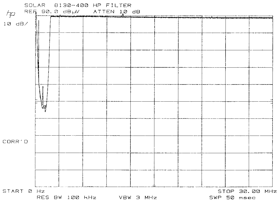
Fig. 1 8130-400 INSERTION LOSS
