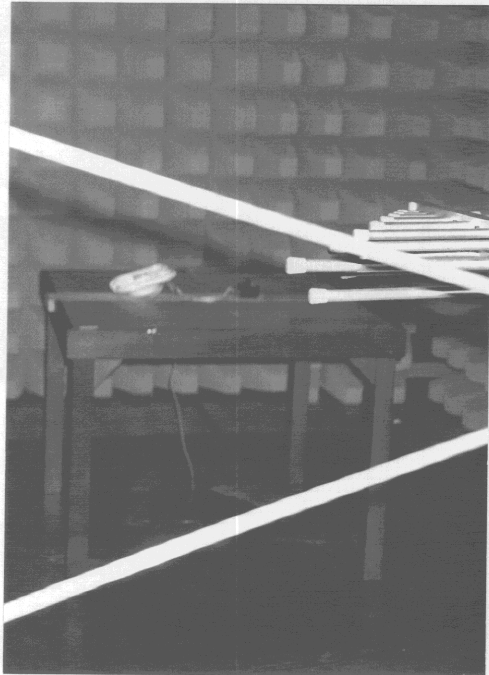
5.1 Radiated emission pre-scan measurement setup in CAC
