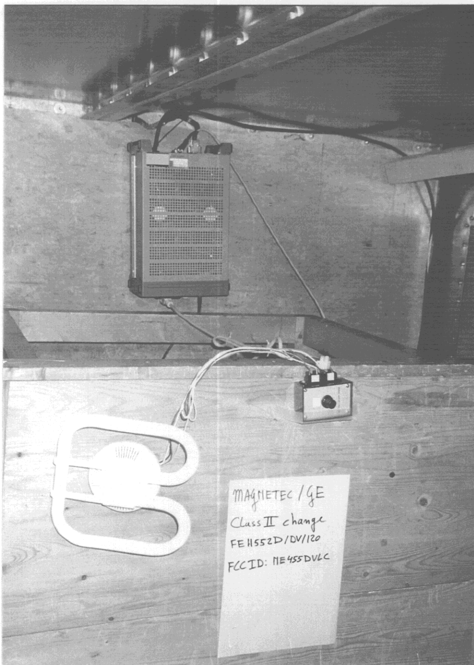
3.1 Conducted emission measurement setup in shielded room
