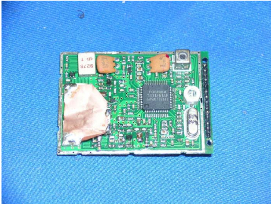
Base Unit Oscillator PCB comp side (View 1)
