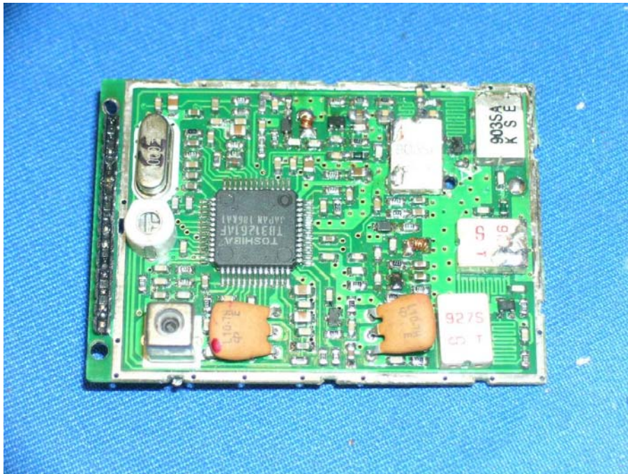
Base Unit Oscillator PCB comp side (View 2)
