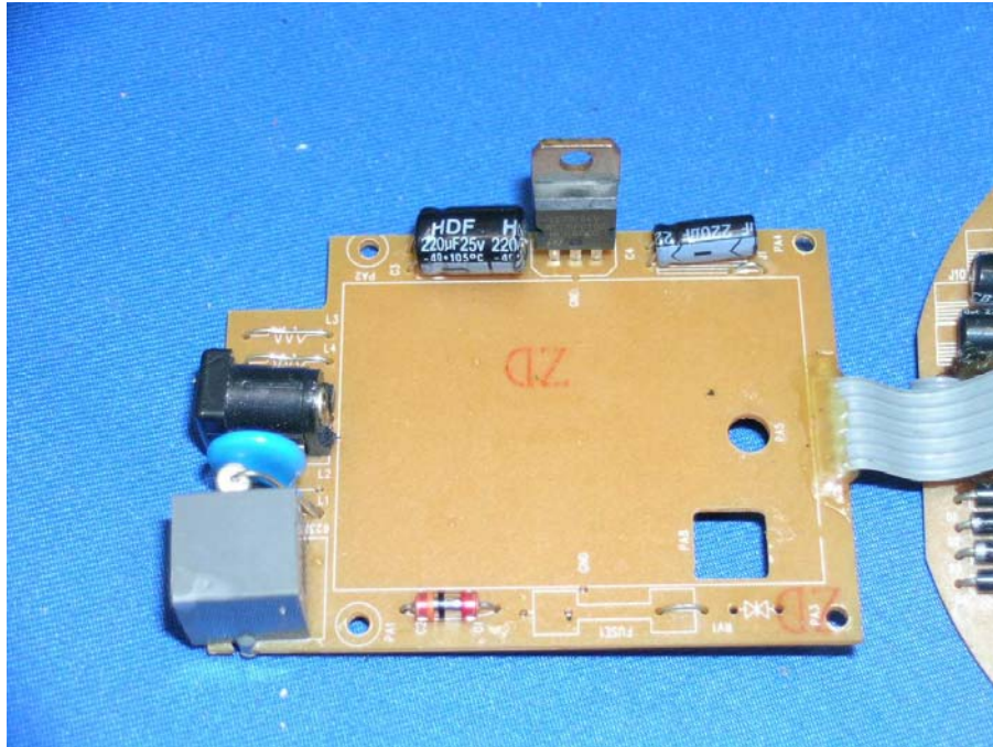
Base another Main PCB comp side
