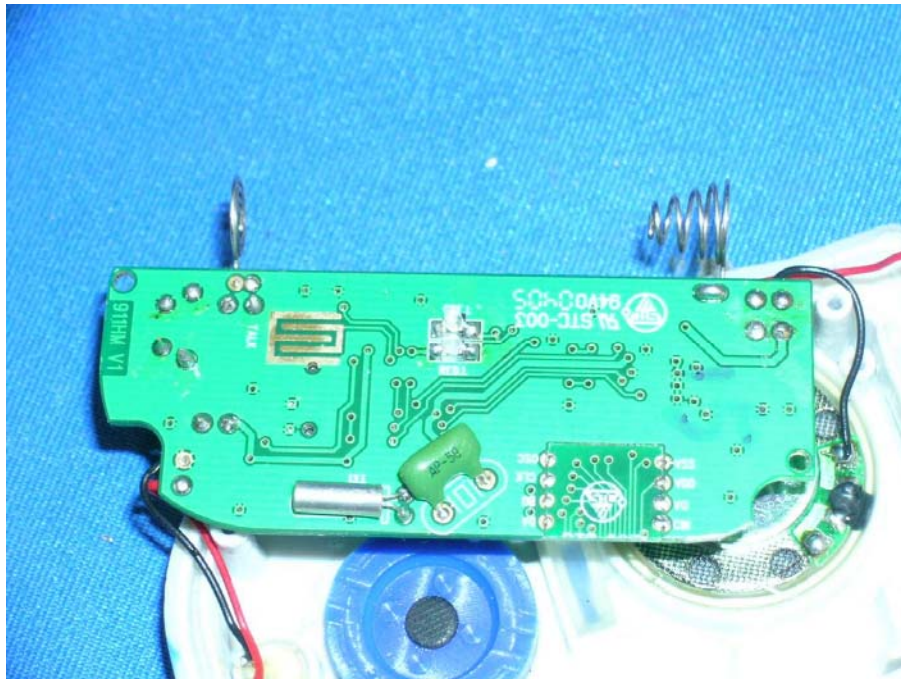
Handset Main PCB solder side
