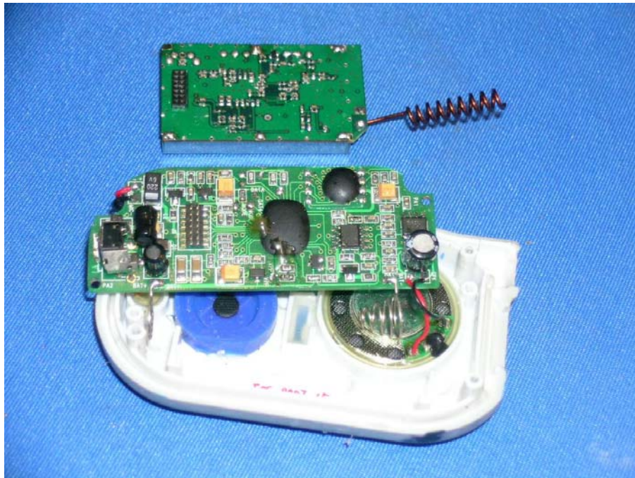
Handset assembly (View 2)
