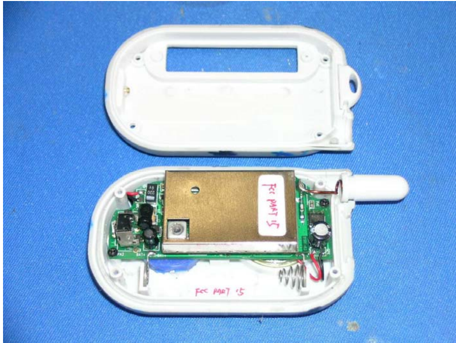
Handset assembly (View 1)
