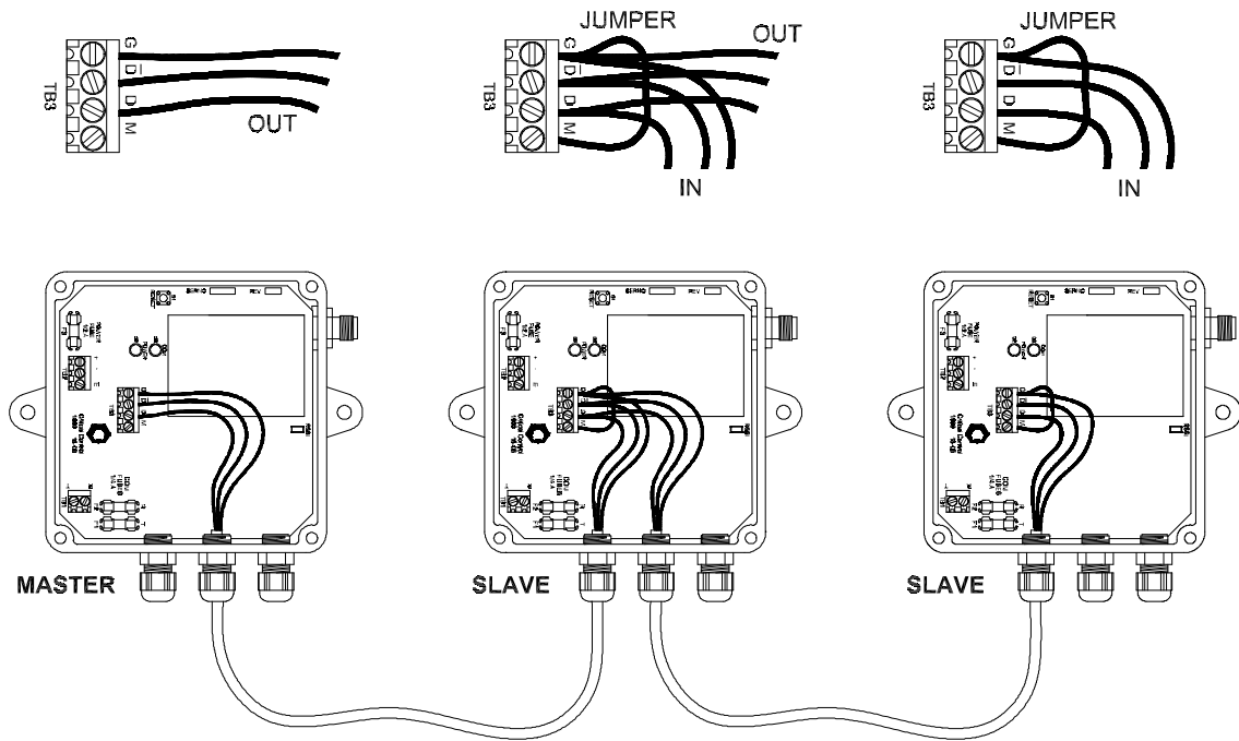
Figure 3: Master – Slave Wiring for Multiple Line Installations
