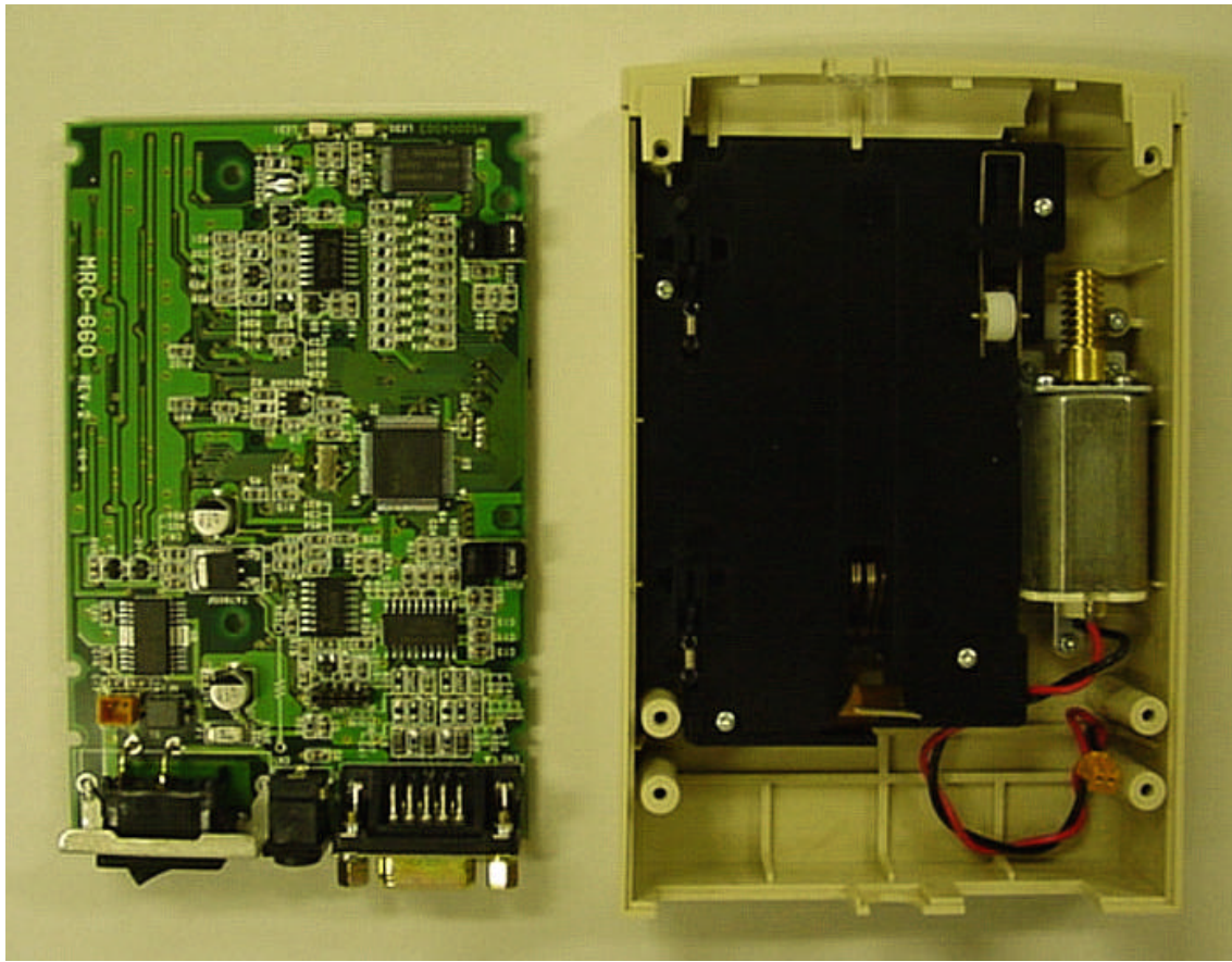
Photo-9 Top Cover & PC Board
