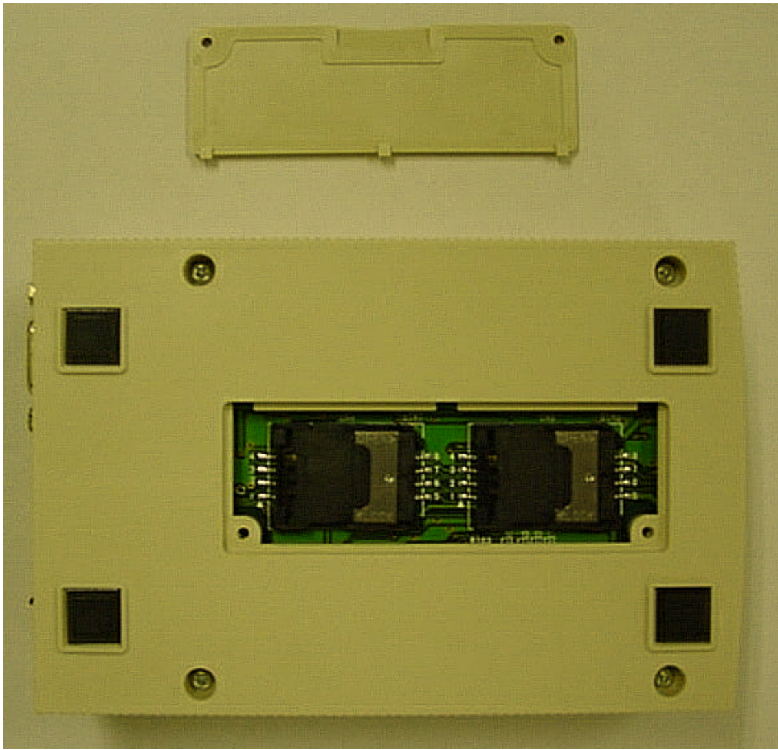
Photo-7 SIM Slot Cover Removed
