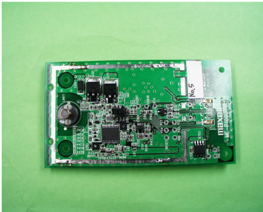
Circuit Board without cover (Rear View)
