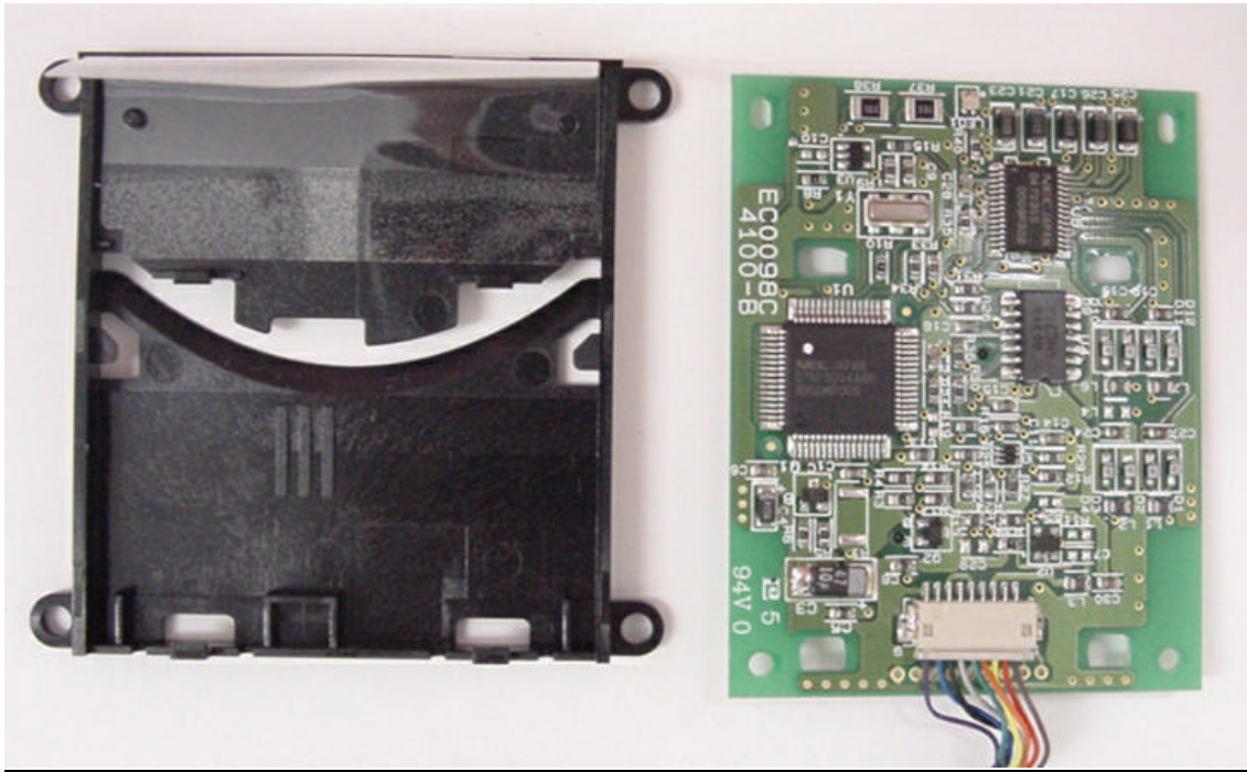
Photo -10 IC Card Connector & PC Board
