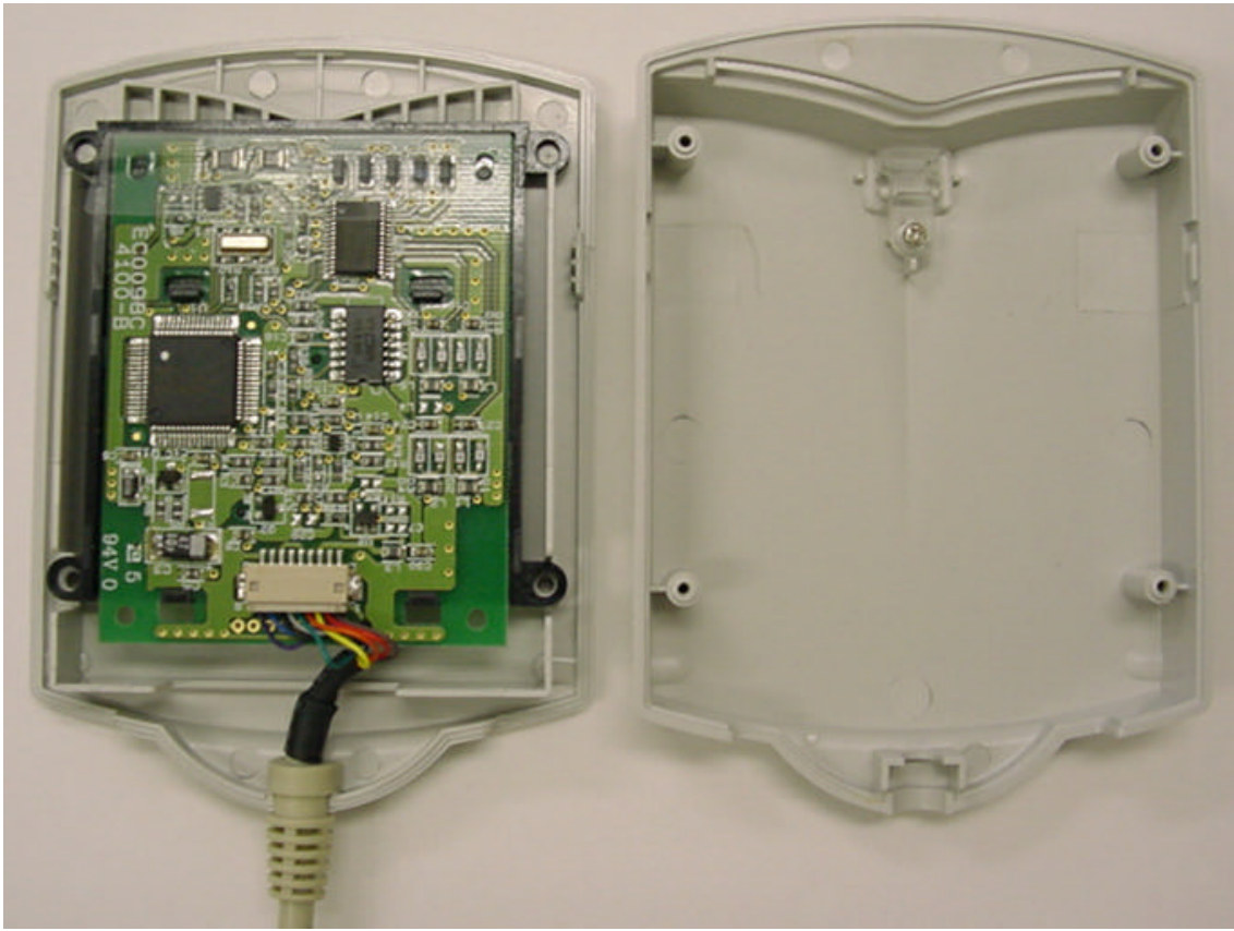
Photo -8 Top Cover Removed
