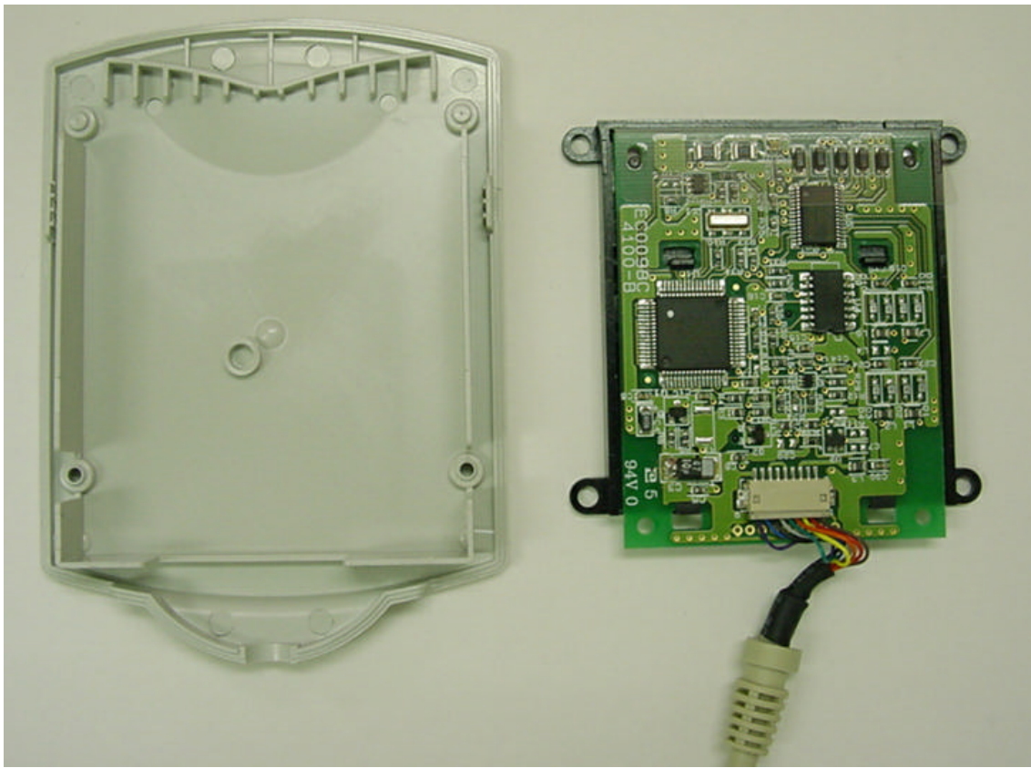
Photo -9 Bottom Cover & PC Board
