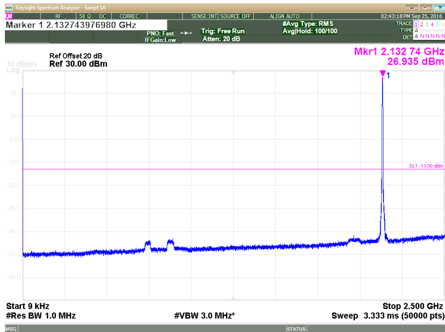
Plot 3.5.3: Spurious Emission Conducted Measurement, AWGN 4.1MHz, Fc = 2132.5 MHz, 9 kHz – 2.5 GHz
