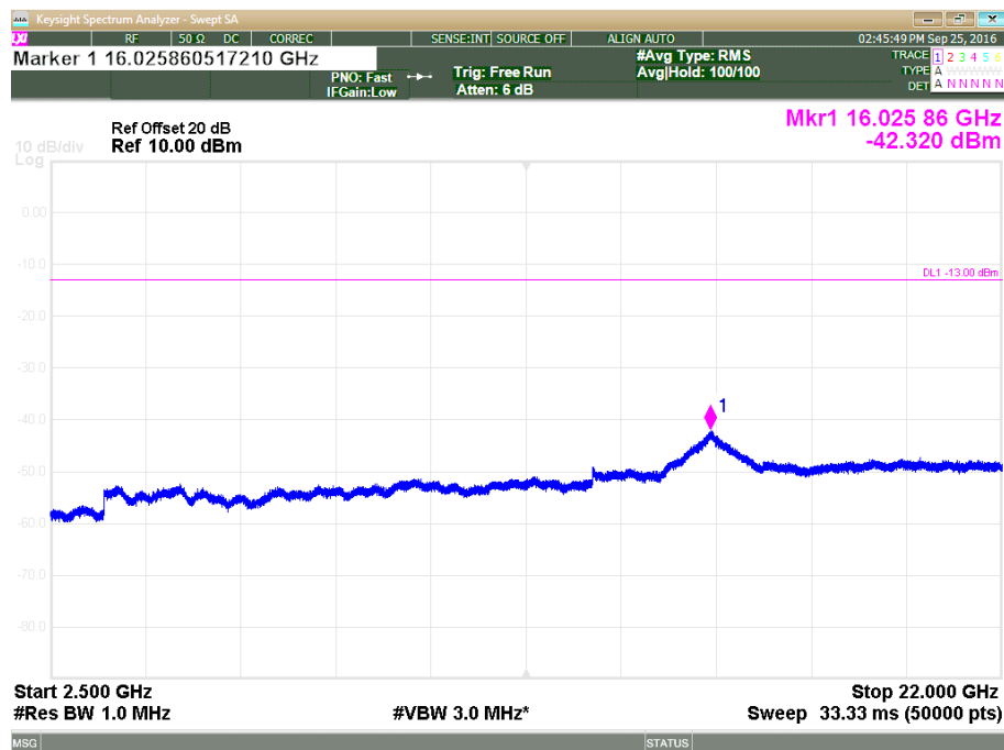
Plot 3.5.4: Spurious Emission Conducted Measurement, AWGN 4.1MHz, Fc = 2132.5 MHz, 2.5 GHz – 22 GHz
