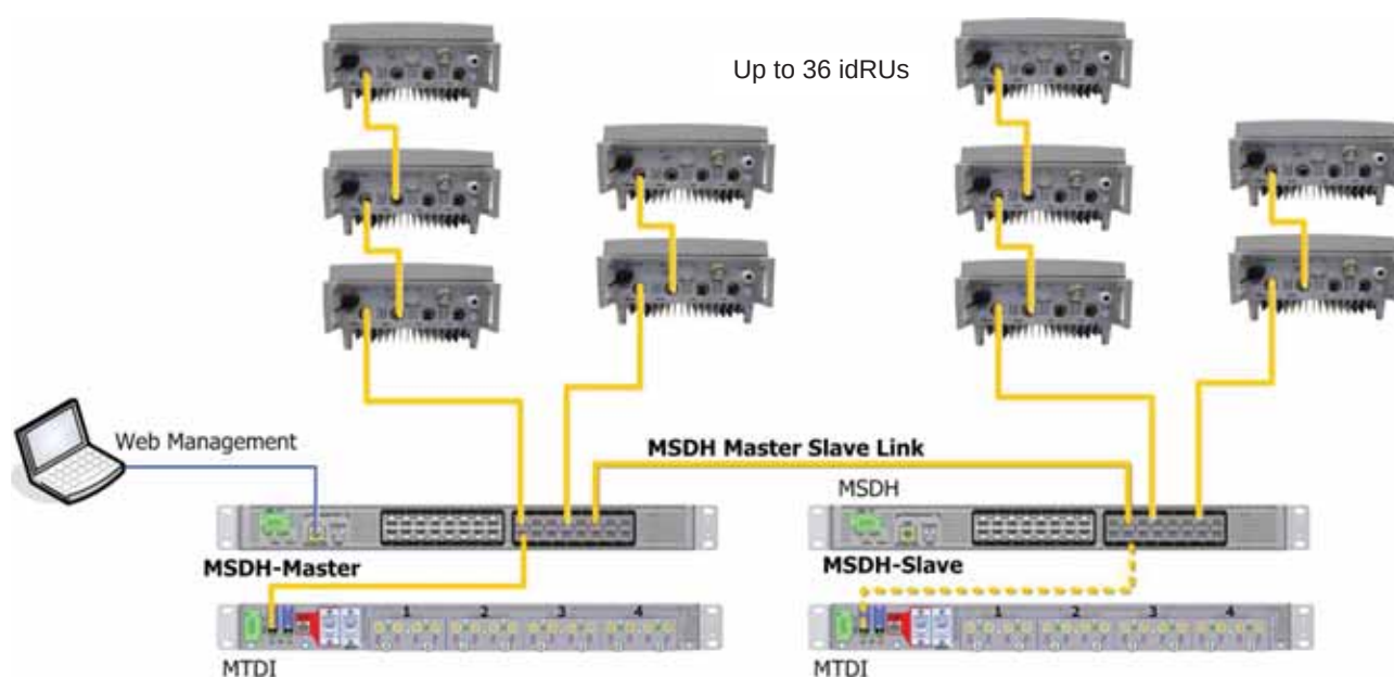
Figure 2-4. MSDH Master Slave Configuration
