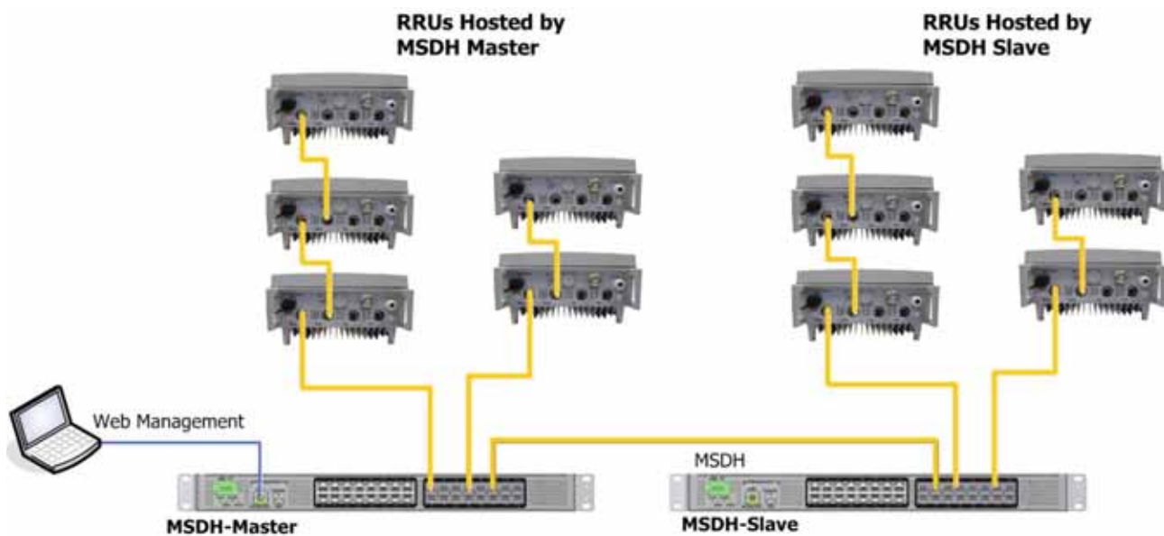
Figure 5-28. Example of Cascaded Repeaters Connections
