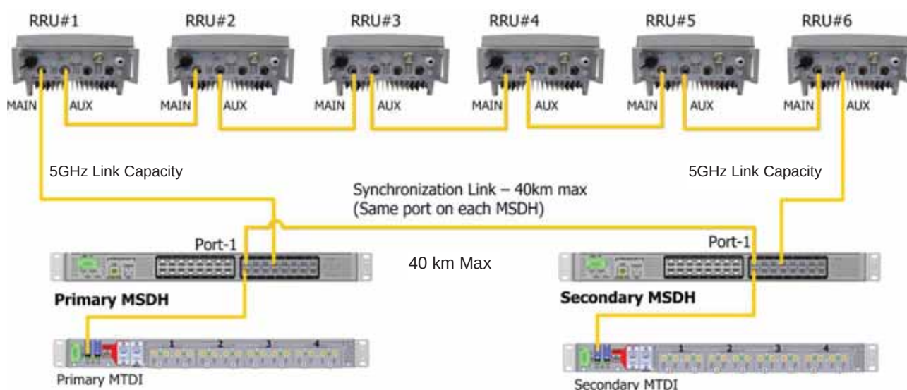
Figure 2-5. Physical Connections of the Redundant idDAS Systems
