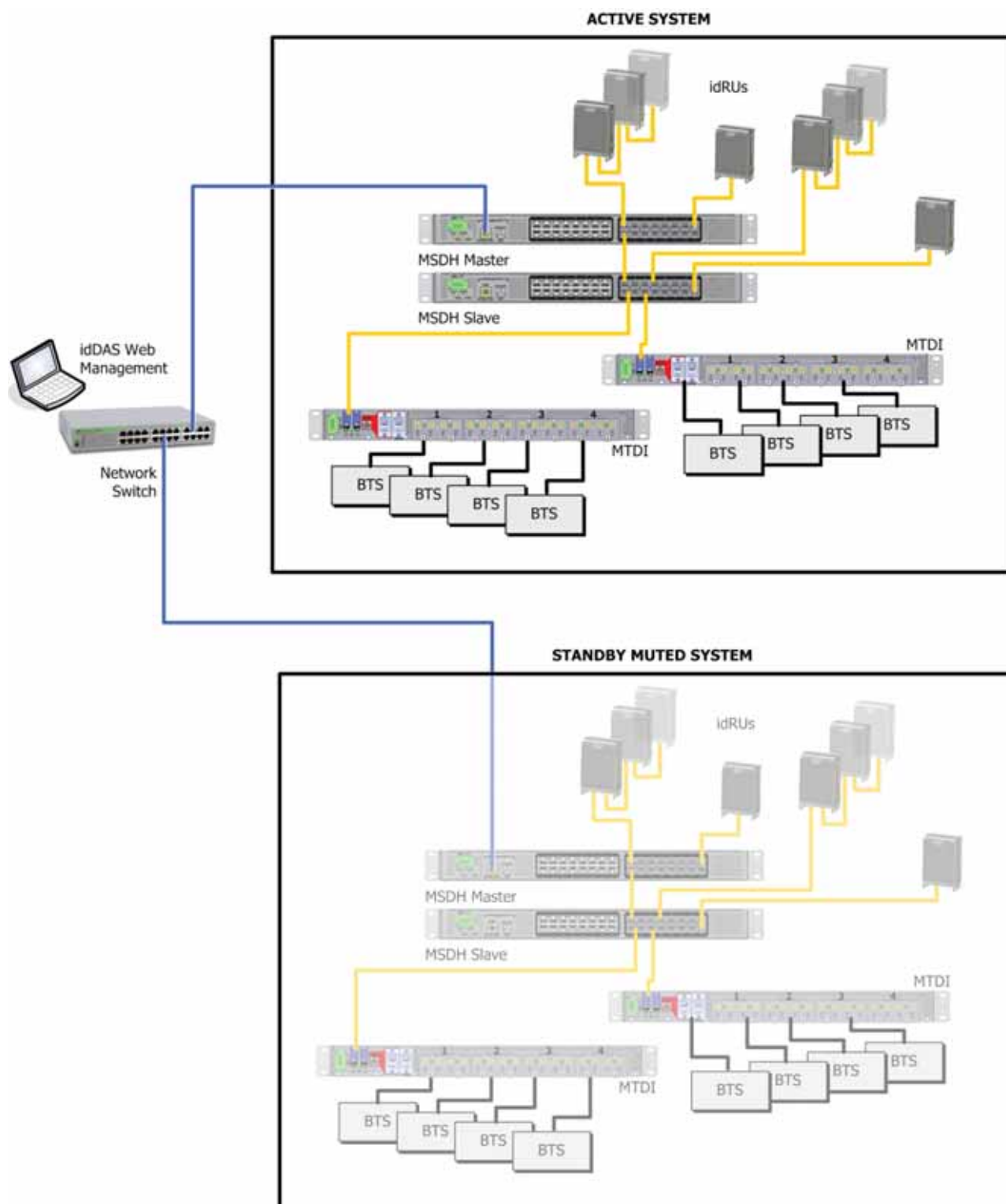
Figure 2-8. Example of Dual-system Redundancy Topology with Master-Slave and Multiple MTDIs
