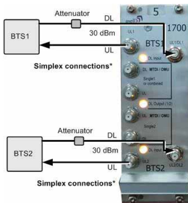
Figure 4-16. BTS Simplex Connections
