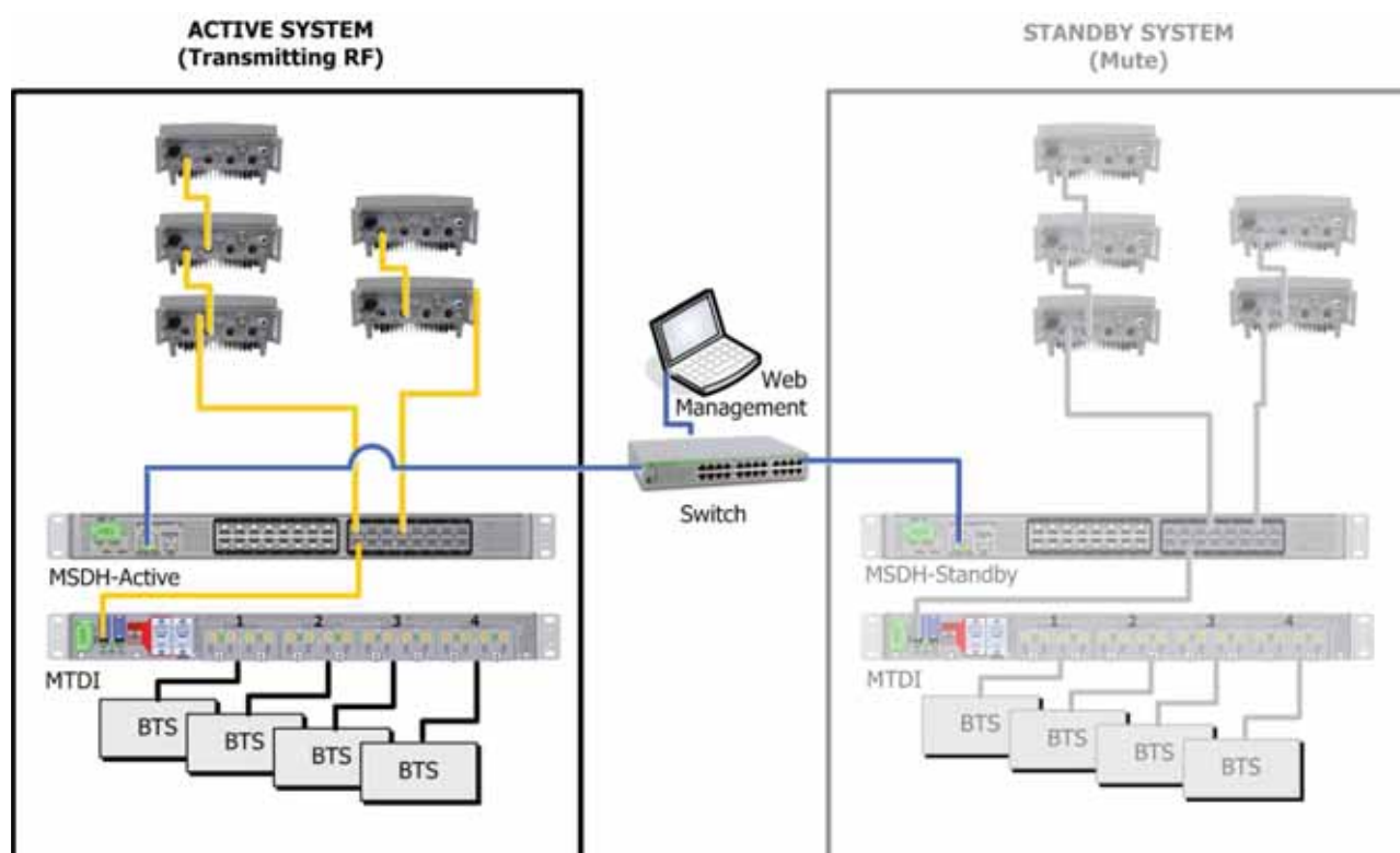
Figure 4-14. idDAS Dual-system Redundancy Topology
