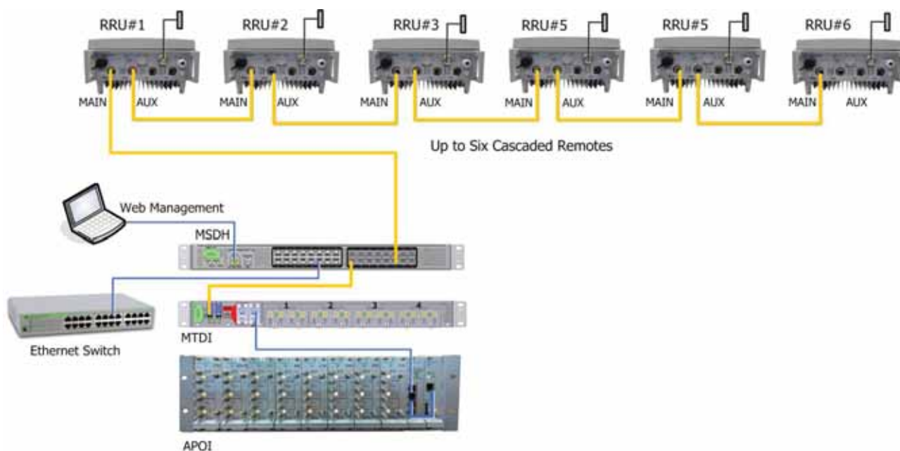
Figure 2-2. Example of a Cascaded idRU Topology
