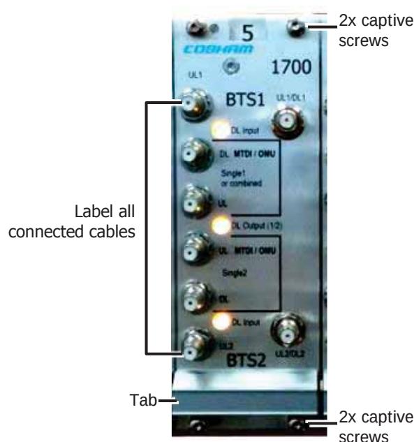
Figure 6-13. Removing RF Modules
