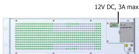
Figure 1-22. APOI 12V DC Power Feed Rear Panel
