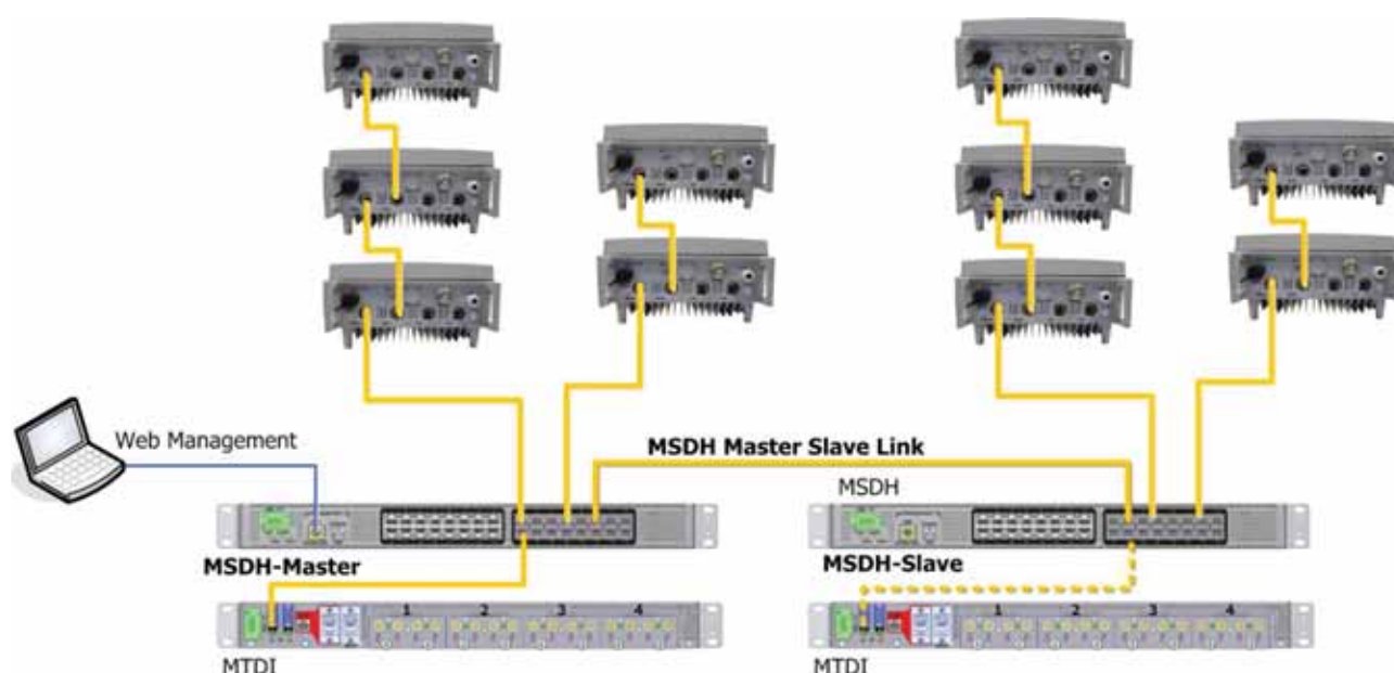
Figure 4-12. Example of a Master Slave Topology
