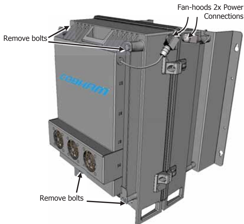
Figure 6-6. Disconnect power Connections and Disassemble Front Fan-hood
