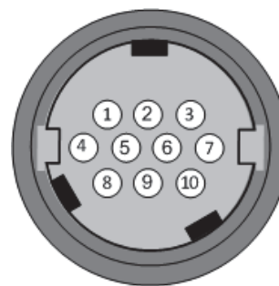
Figure 5-37. Alarms 10 Pin Circular Connector
