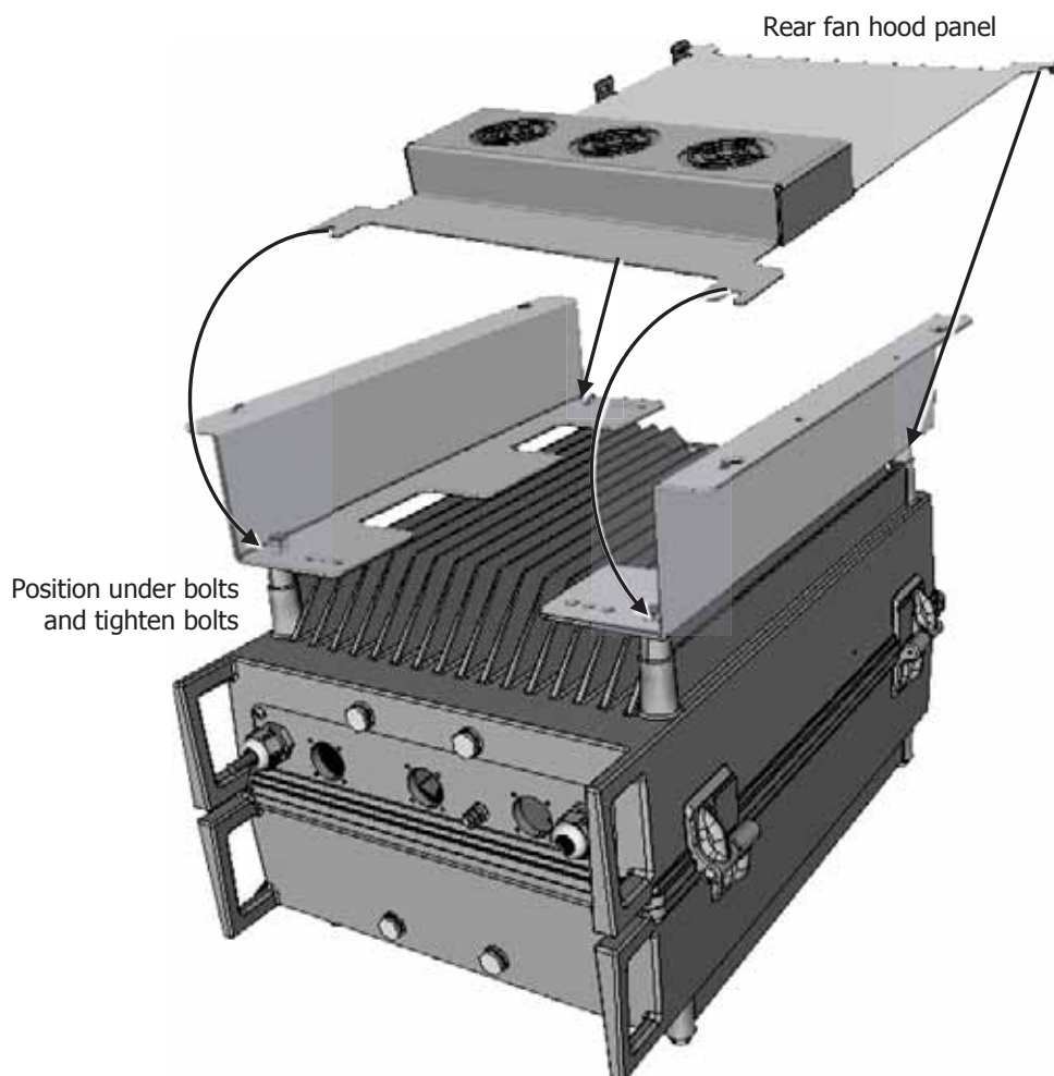
Figure 5-9. Assembling Rear Fan Hood Panel
