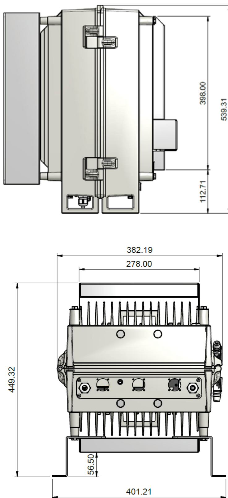
Figure 5-7. idRU with Fan Hood Assembly Dimensions
