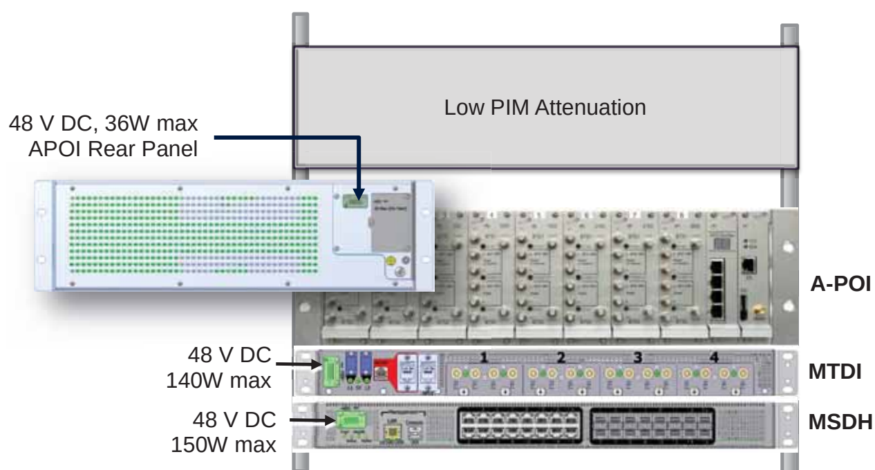
Figure 4-4. APOI, MTDI and MSDH 48 V DC Power Connections
