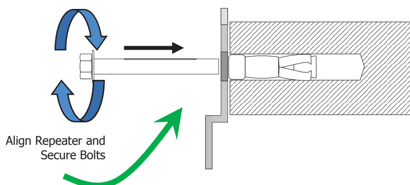
Figure 5-20: Mount Repeater
