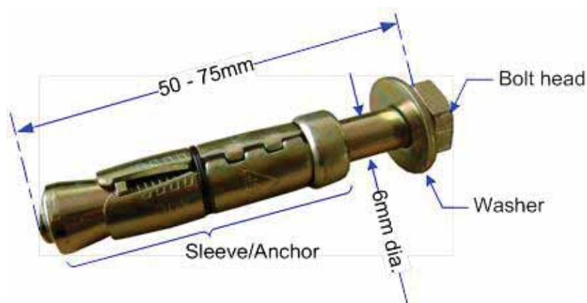
Figure 5-15. M6 Rawlbolt – recommended for wall mount.
