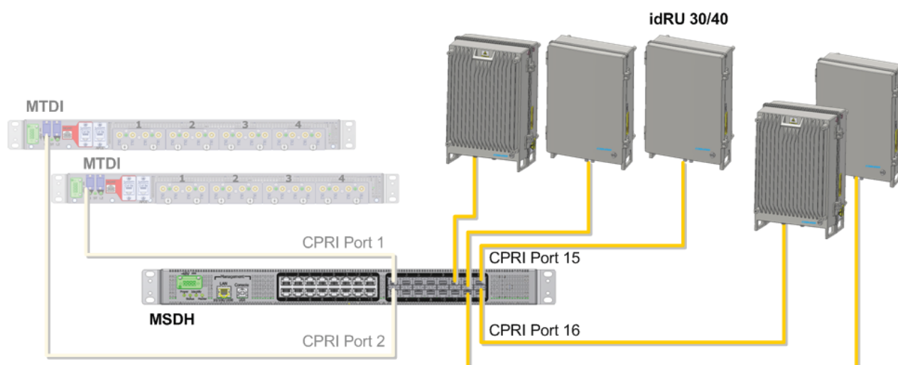
Figure 4-21. Example of idRU to MSDH Connections
