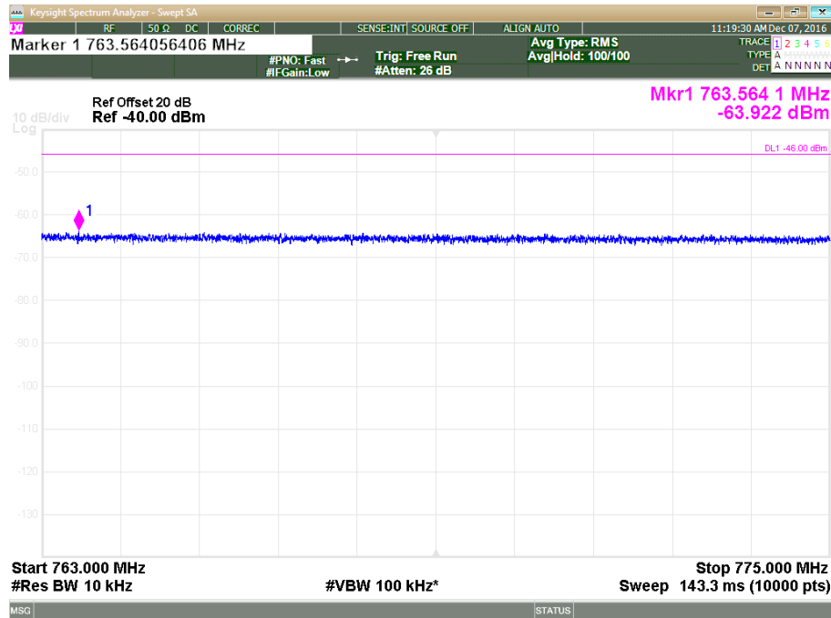
Plot 3.5.3: Spurious Emission Conducted Measurement, AWGN 4.1MHz, Fc = 748.5 MHz, 763 MHz – 775 MHz
