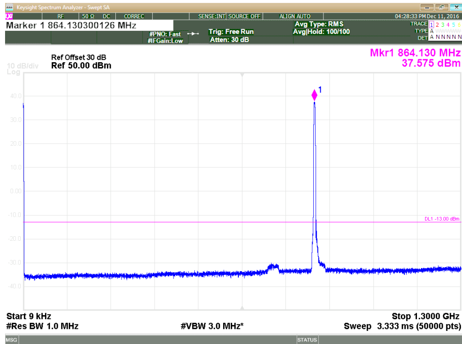
Plot 3.5.7: Spurious Emission Conducted Measurement, AWGN 4.1MHz, Fc = 864.500 MHz, 9.0 KHz – 1.3 GHz
