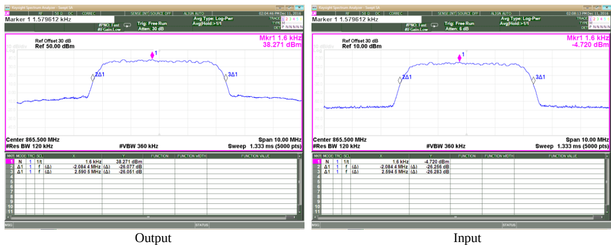
Plot 3.2.2: Input-versus-output signal comparison, AWGN 4.1MHz
