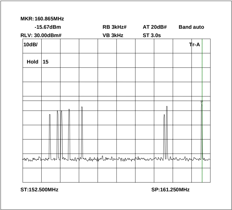
Scan plot showing amplifiers channels
