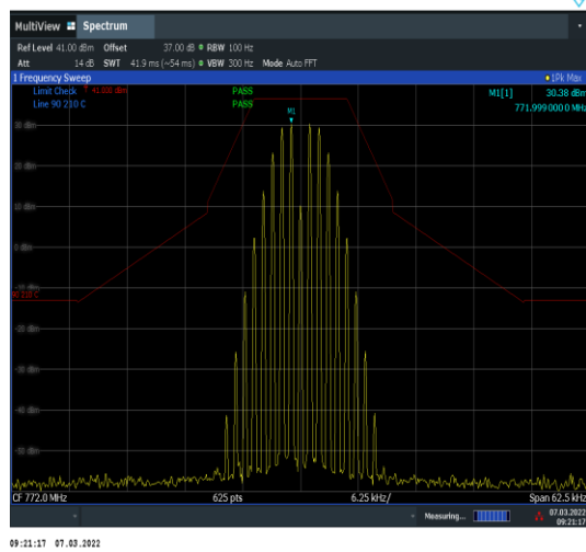
P25 C4FM Mask C @ AGC+3 dB
