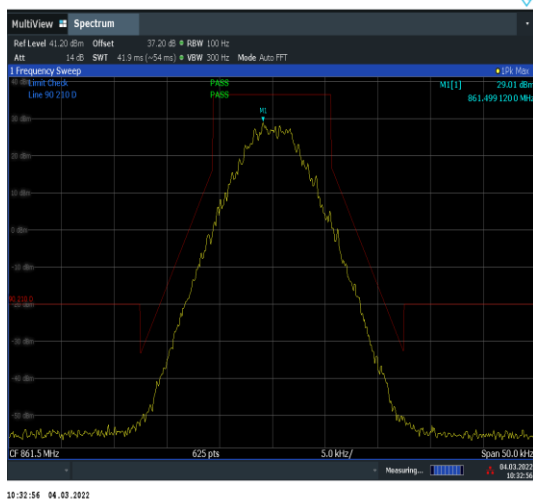
P25 C4FM Mask D @ AGC+3 dB
