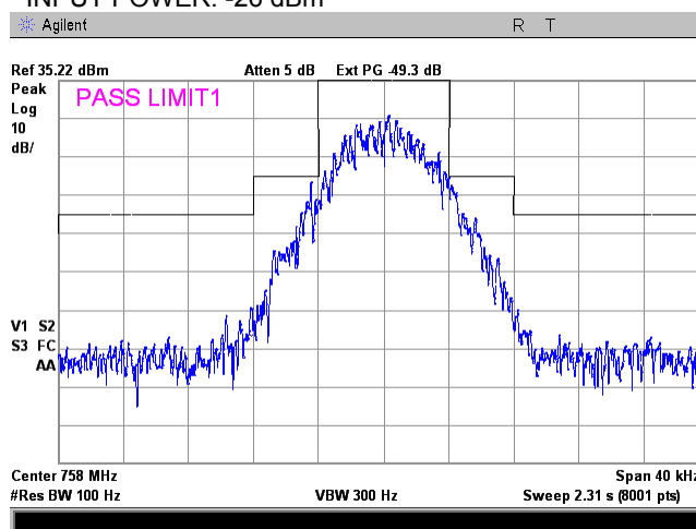
Plot 7.3.14 Emission mask test result at mid frequency carrier, Port 1
