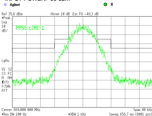
Plot 7.3.22 Emission mask test result at low frequency carrier, Port 2
