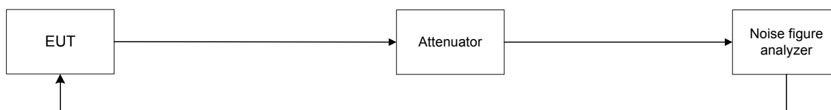
Figure 7.7.1 Noise figure test setup
