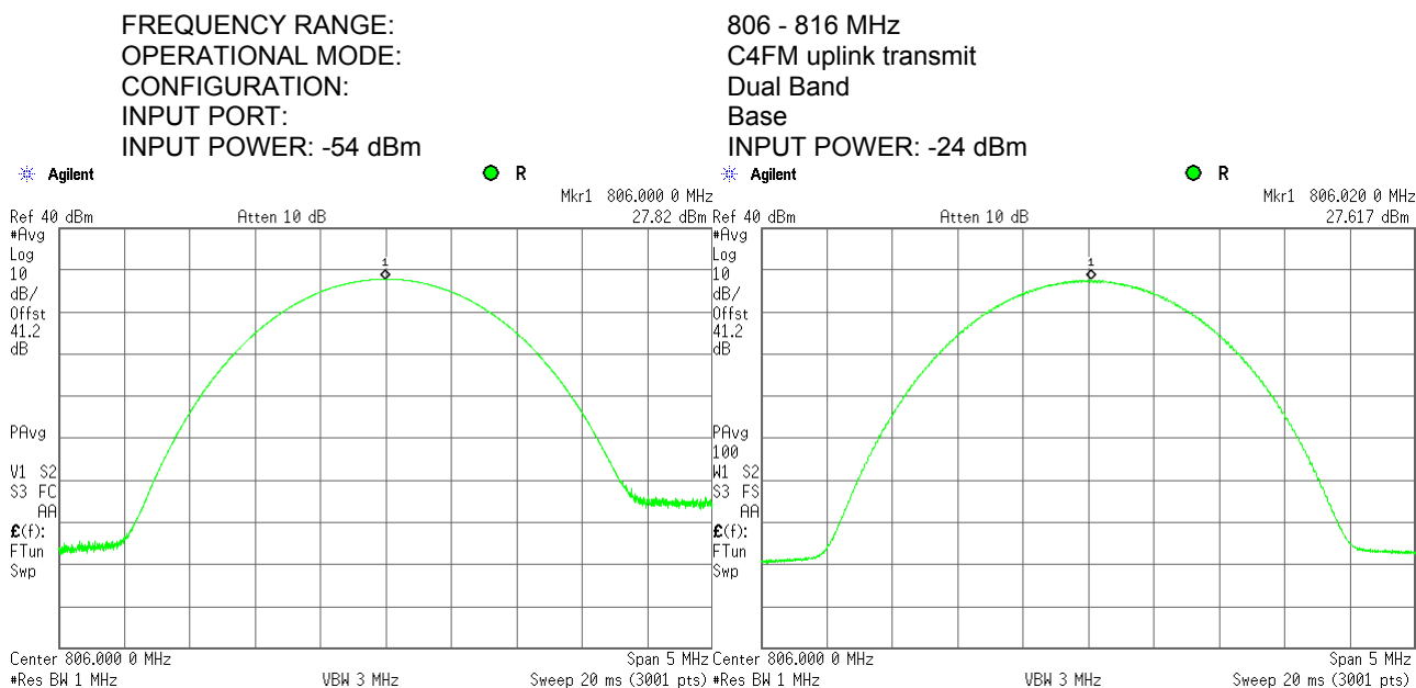
Plot 7.1.10 RF output power measurements at low frequency carrier, Port 2
