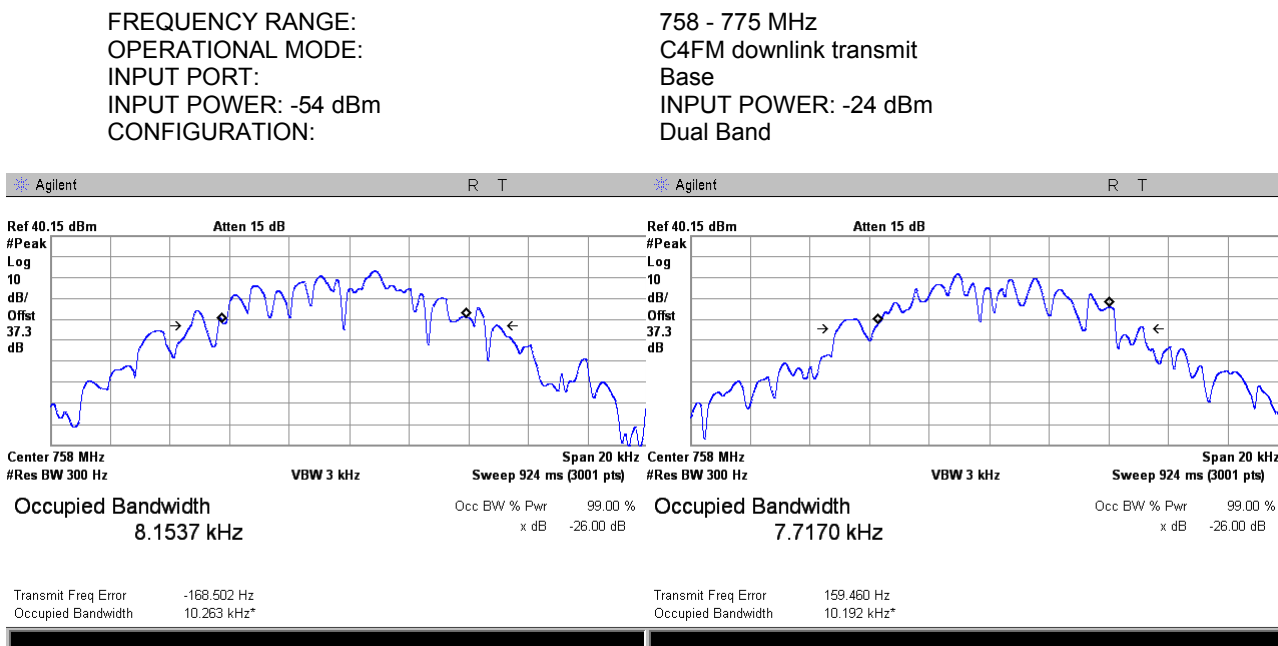
Plot 7.2.1 Occupied bandwidth test result at low frequency carrier, Port 1
