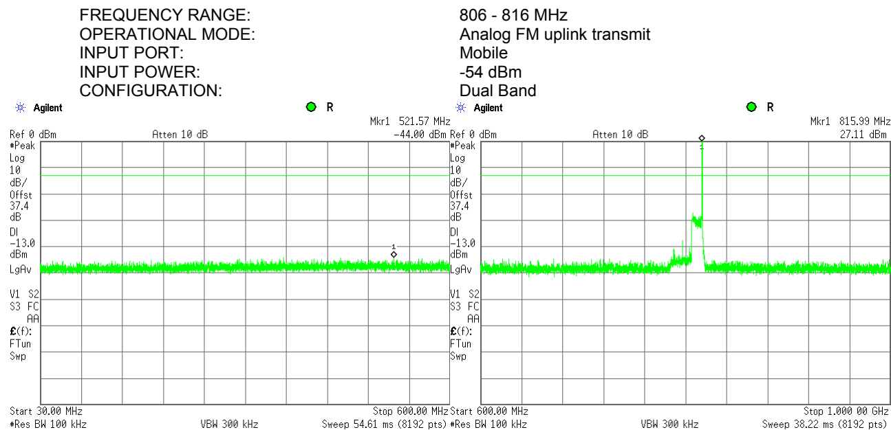
Plot 7.6.141 Spurious emission measurements in 30.0 - 1000 MHz range at high carrier frequency
