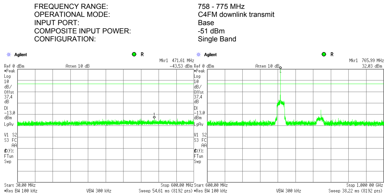
Plot 7.6.8 Spurious emission measurements in 30.0 - 1000 MHz range at mid carrier frequency
