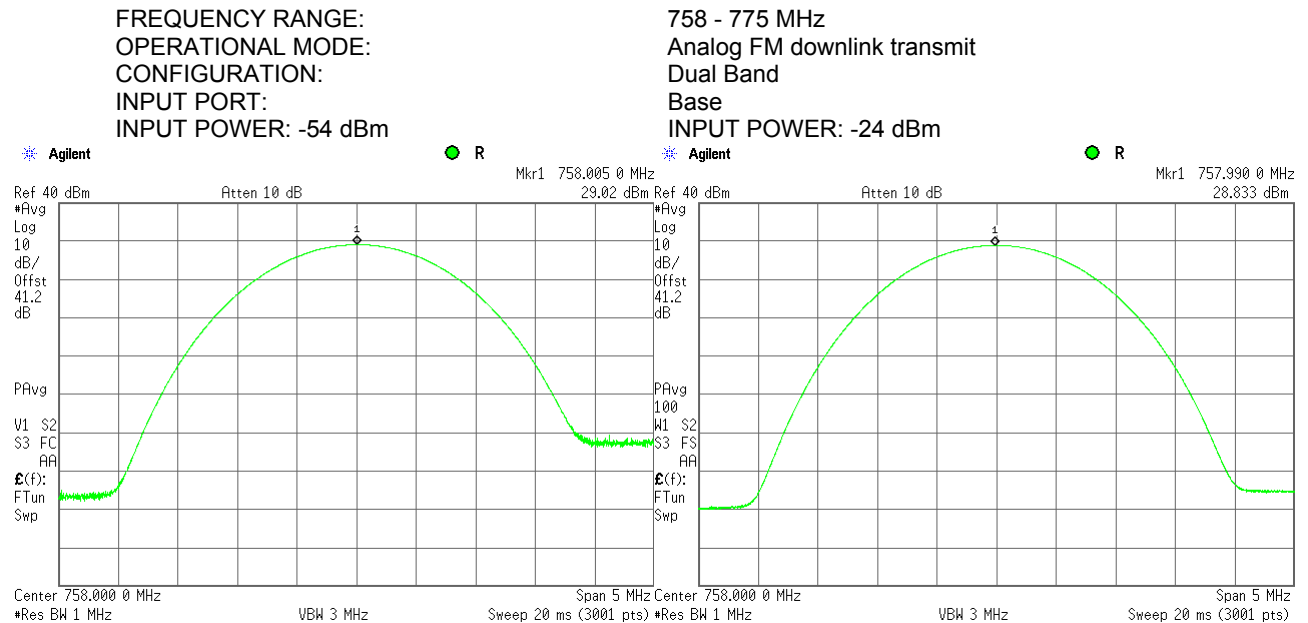
Plot 7.1.37 RF output power measurements at low frequency carrier, Port 1
