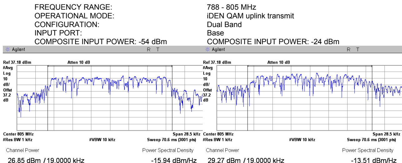
Plot 7.1.24 RF output power measurements at highfrequency carrier, Port 2
