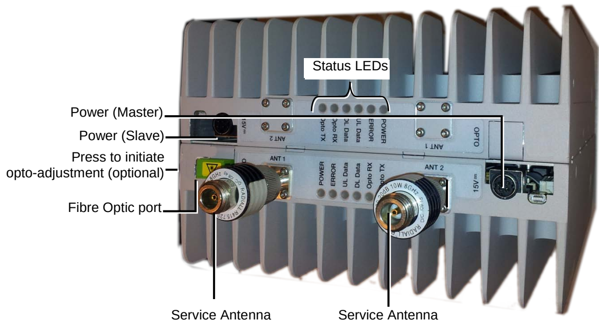
Figure 1-3: MBF-20 Quad-Band Front Panel
