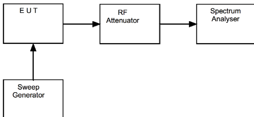
Figure v Test Setup
