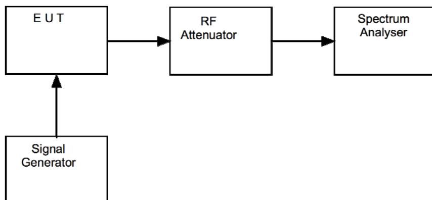
Figure vi Test Setup
