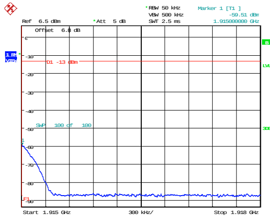
1850-1915MHz 1 x AWGN AGC +3dB upper
