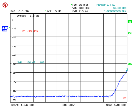
1850-1915MHz 1 x AWGN ≤ AGC lower
