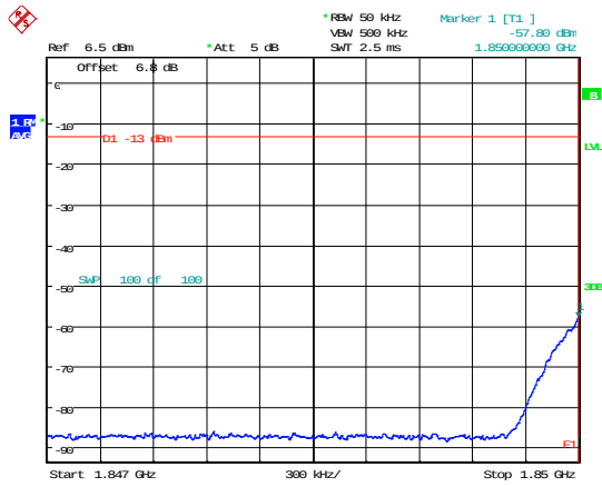
1850-1915MHz 1 x AWGN AGC +3dB lower
