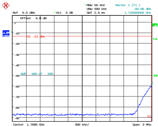
1710-1755MHz 1 x AWGN \leq AGC lower
