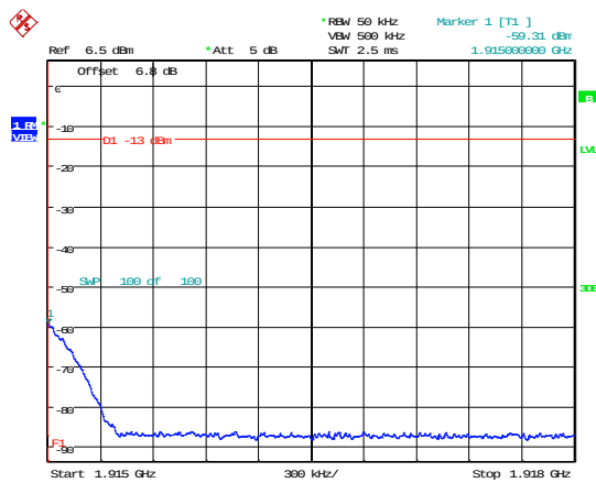
1850-1915MHz 1 x AWGN ≤ AGC Upper
