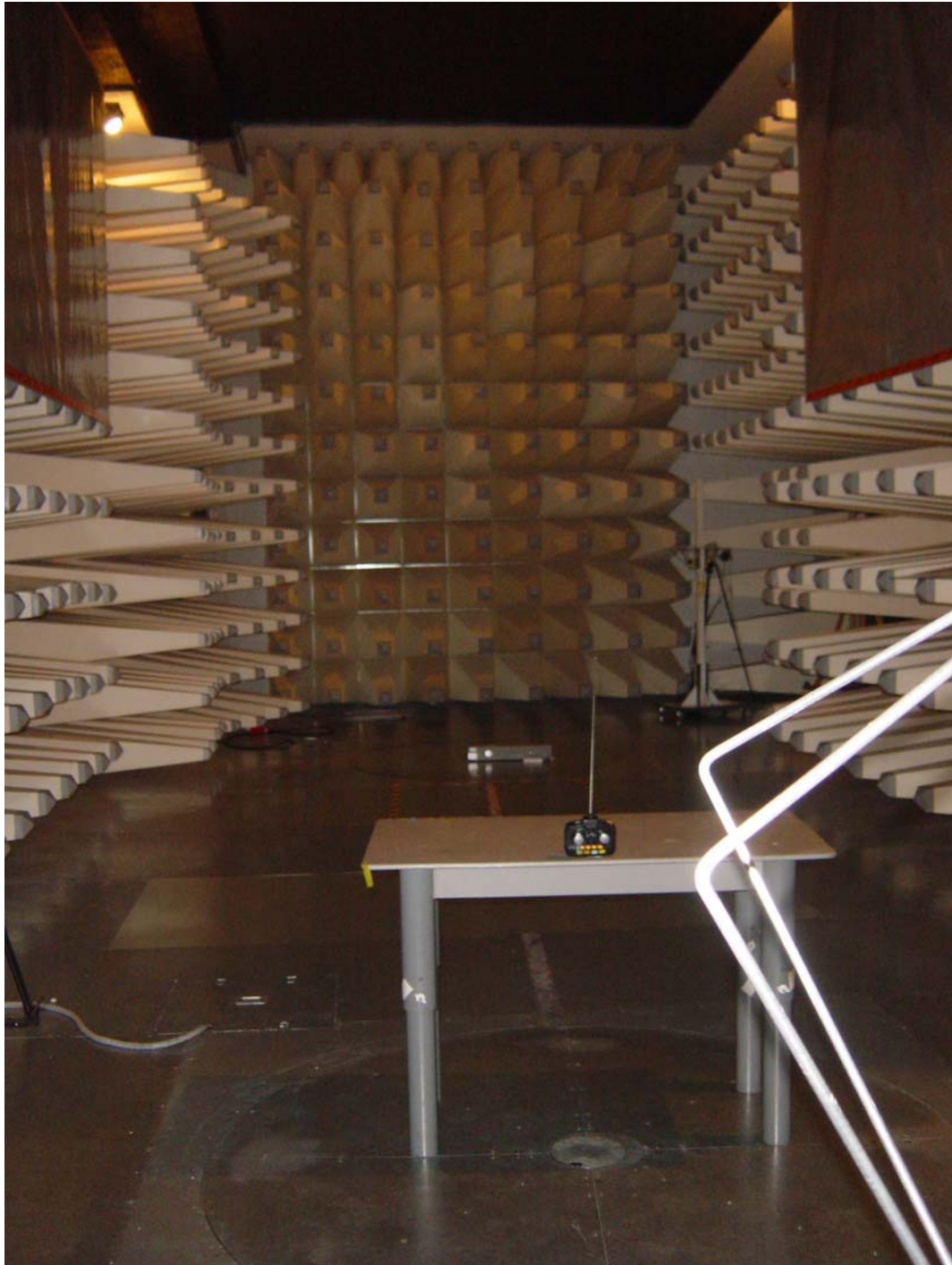
Set-up for Radiation Emission ( Transmitter)
