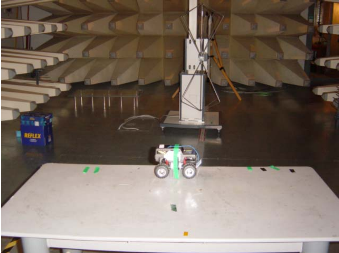
Set-up for Radiation Emission (Receiver)
