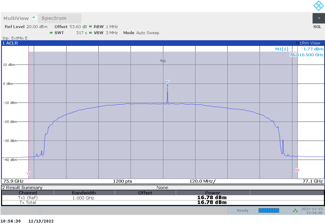
Plot no. 3: Mean Power EIRP, RMS detector / Channel Power, DMP12
